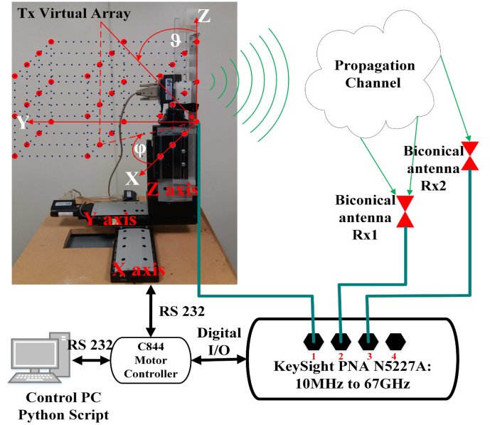
Fig. 1: Measurement Setup.
