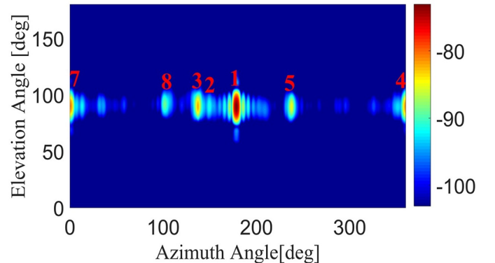
Fig. 7: Elevation and azimuth power angle spectrum for the LOS scenario. Color bar units in dB.
