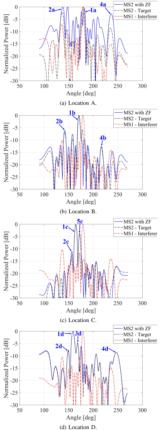
Fig. 11: PAP with ZF-BF at 28 GHz for MS2 in comparison to the PAP for MS2 and MS1 without ZF-BF. The MPCs labels correspond to paths identified in Fig. 9.
