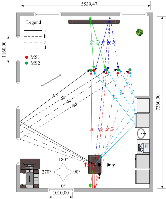
Fig. 10: Trajectory of MPCs in relation to the room geometry for the multi-user scenario in LOS conditions. Propagation paths to each location are represented by different lines as shown in the legend. Dimensions are in millimeters.
