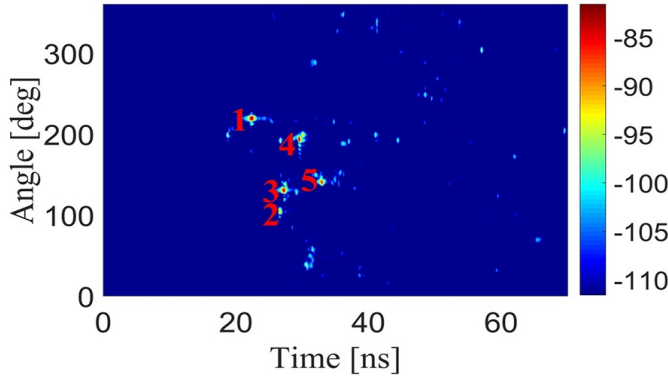
Fig. 5: PADP for the OLOS scenario. Color bar units in dB.
