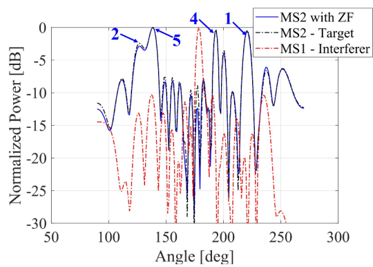
(b) PAP with ZF-BF at 28 GHz for MS2 in comparison to the PAP for MS2 and MS1 without ZF-BF.
