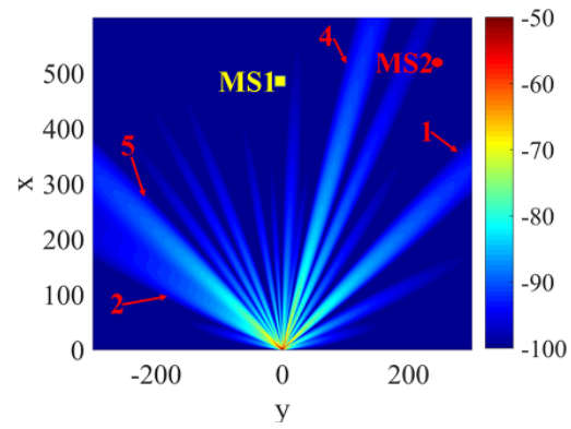
(a) Field pattern distribution with MS2 the target user and MS1 the interfering user. x and y denote the location coordinates with units \lambda and the colour bar units in dB.
