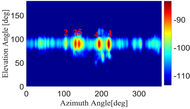
Fig. 8: Elevation and azimuth power angle spectrum for the OLOS scenario. Color bar units in dB.
