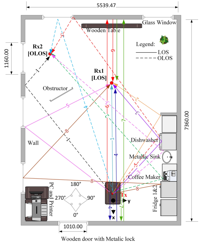
Fig. 6: Trajectory of the MPCs in relation to the room geometry for the LOS and OLOS scenario. The dashed lines represent the MPCs corresponding to the OLOS scenario. Dimensions are in millimeters.
