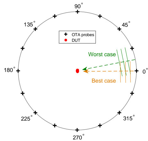
Fig. 2. The OTA probe configuration for the simulation in Section IV. “Best case” denotes the impinging angle at 0°, and “Worst case” the impinging angle at 11.25°.
