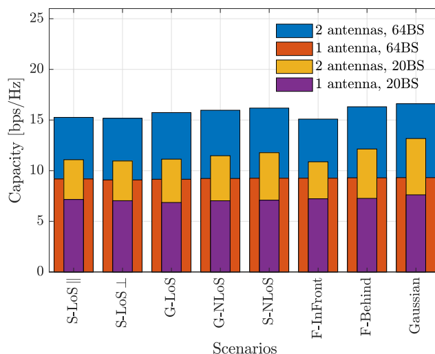
FIGURE 6. DPC capacity averaged over users with 1 and 2 antennas at 10dB, C2D array.
