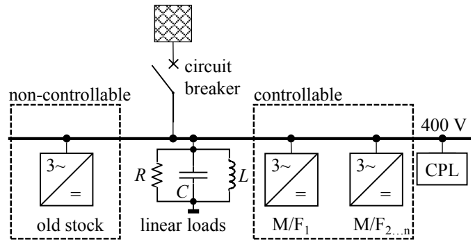
Fig. 1. Low-voltage islanded grid with a connection to the medium voltage grid that can be disconnected by a circuit breaker. Several linear loads ( RLC ) and nonlinear loads (constant power load, CPL) are assumed. Controllable (Master M / Follower F) and non-controllable ( old stock ) inverters are connected to the islanded grid.
