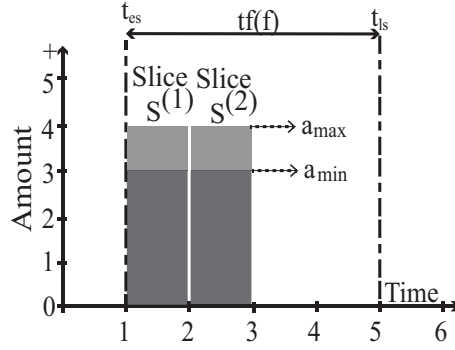
Fig. 1.1: Illustration of a flex-offer
