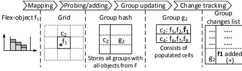
Fig. 3.6: Processing the addition of a flex-object in the grouping phase
