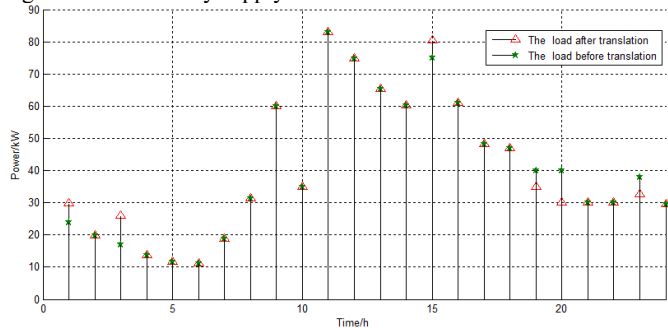
Fig.6. Shifting loads.
