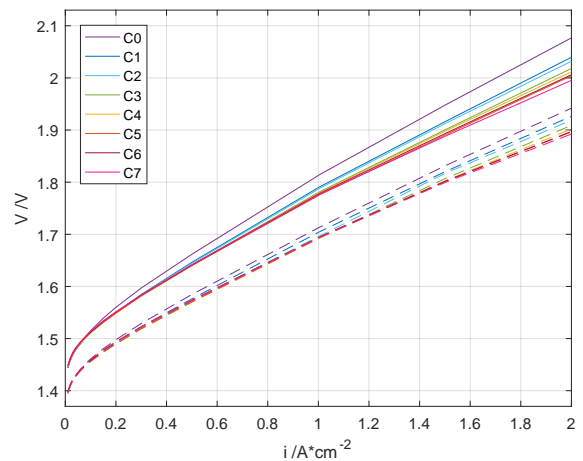
Figure 5: Polarization curves for all compressions at 60^\circ\text{C} (solid) and 80^\circ\text{C} (dashed)
