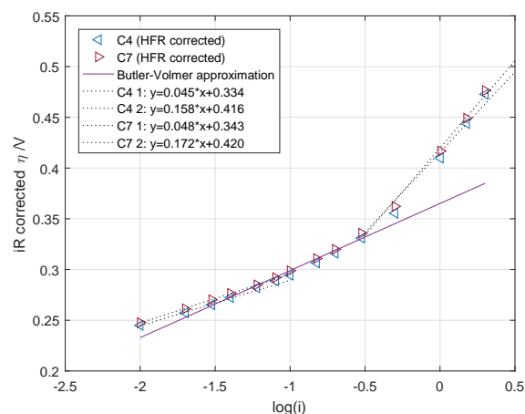
(b) Comparison between C4 and C7 (HFR-correction)
