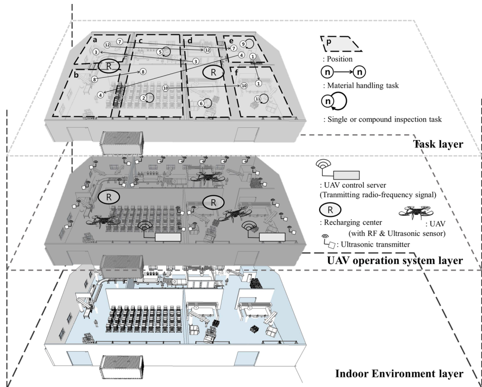
Fig. 1 Architecture of indoor UAV system
