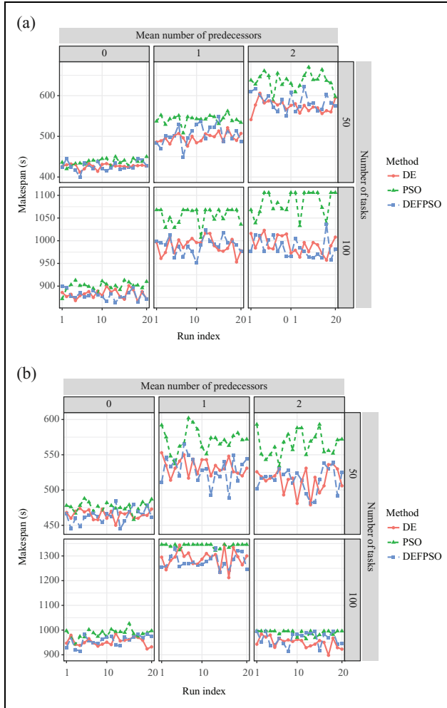
Figure 3. Makespan of schedules for laboratory scale (a) and industrial scale (b) data sets with DE, PSO, and DEFPSO. DE: differential evolution; PSO: particle swarm optimization; DEFPSO: DE-fused PSO.
