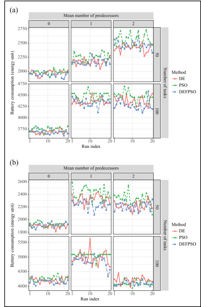
Figure 4. Total battery consumption of schedules for laboratory scale (a) and industrial scale (b) data sets with DE, PSO, and DEFPSO. DE: differential evolution; PSO: particle swarm optimization; DEFPSO: DE-fused PSO.
