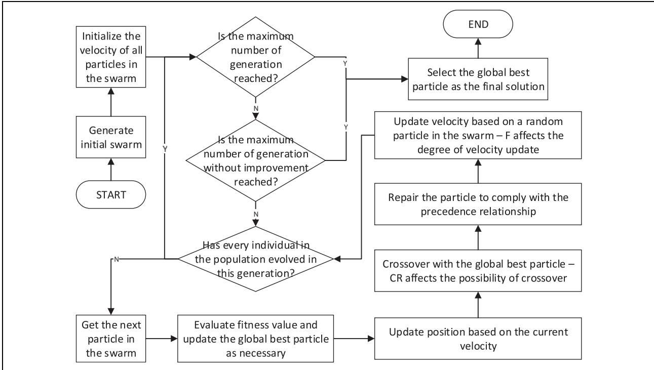
Figure 2. Flowchart of DEFPSO algorithm. DEFPSO: differential evolution-fused particle swarm optimization.
