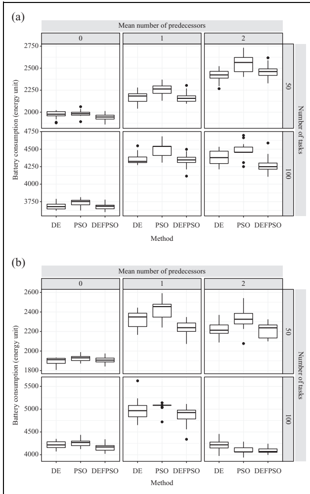
Figure 7. Boxplot of battery consumption of schedules for laboratory scale (a) and industrial scale (b) data sets in connection with the results in Figure 4.
