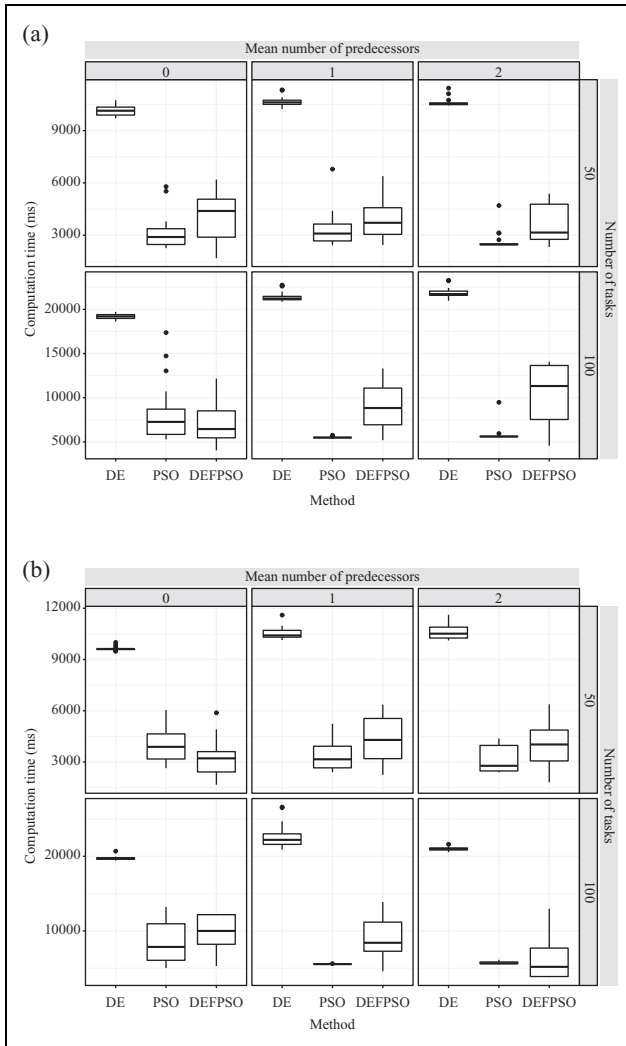
Figure 1C. Computation time of schedules for laboratory scale (a) and industrial scale (b) data sets with DE, PSO, and DEFPSO. DE: differential evolution; PSO: particle swarm optimization; DEFPSO: DE-fused PSO.
