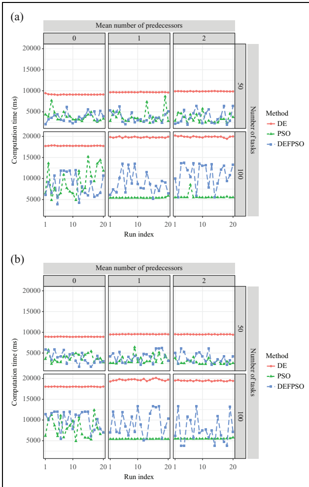
Figure 5. Computation time of schedules for laboratory scale (a) and industrial scale (b) data sets with DE, PSO, and DEFPSO. DE: differential evolution; PSO: particle swarm optimization; DEFPSO: DE-fused PSO.
