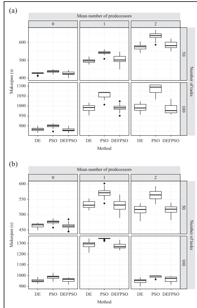
Figure 6. Boxplot of makespan of schedules for laboratory scale (a) and industrial scale (b) data sets in connection with the results in Figure 3.
