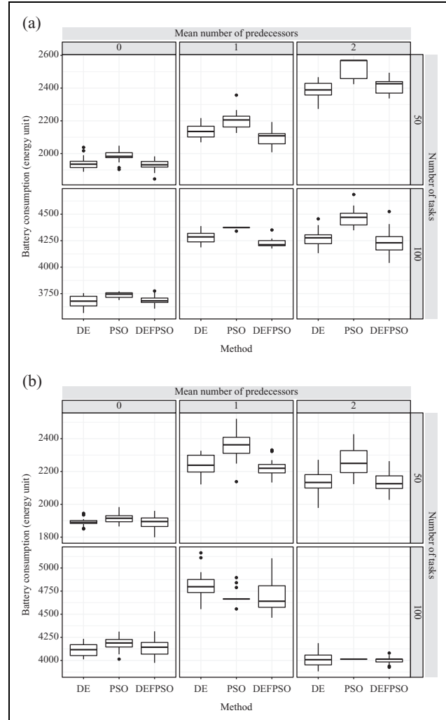
Figure 1B. Battery consumption of schedules for laboratory scale (a) and industrial scale (b) data sets with DE, PSO, and DEFPSO. DE: differential evolution; PSO: particle swarm optimization; DEFPSO: DE-fused PSO.
