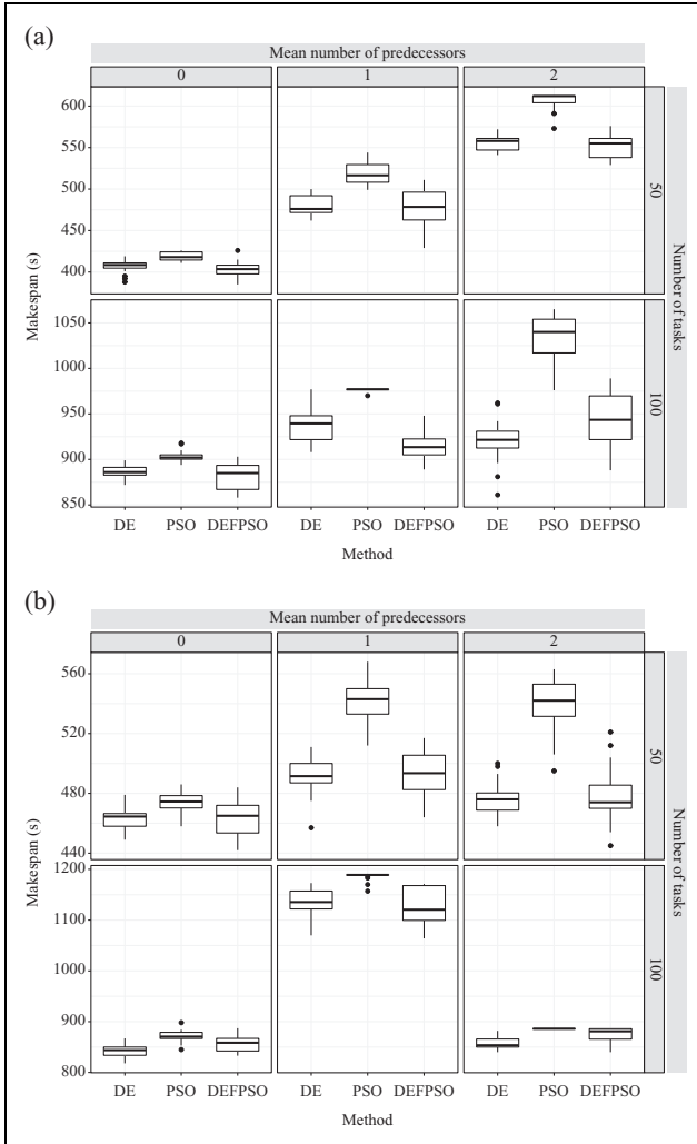
Figure 1A. Makespan of schedules for laboratory scale (a) and industrial scale (b) data sets with DE, PSO, and DEFPSO. DE: differential evolution; PSO: particle swarm optimization; DEFPSO: DE-fused PSO.
