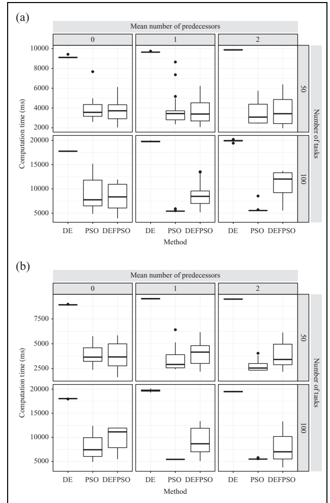
Figure 8. Boxplot of computation time of schedules for laboratory scale (a) and industrial scale (b) data sets in connection with the results in Figure 5.
