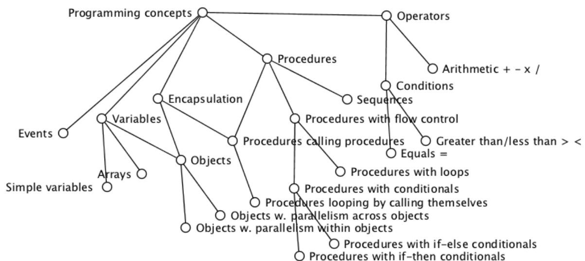
Figure 1. A concept specialisation map (CSM) showing all the programming concepts identified by Allsopp & Ejsing-Duun (2016)
