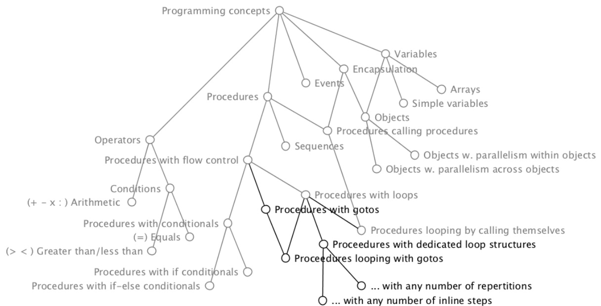
Figure 4. The updated CSM with the new specialisation and programming concepts emphasized
