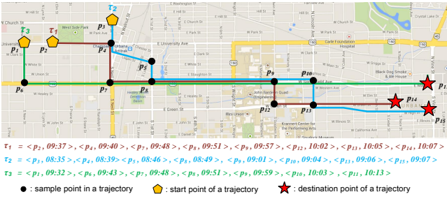
Figure 1: TS-Join Example
