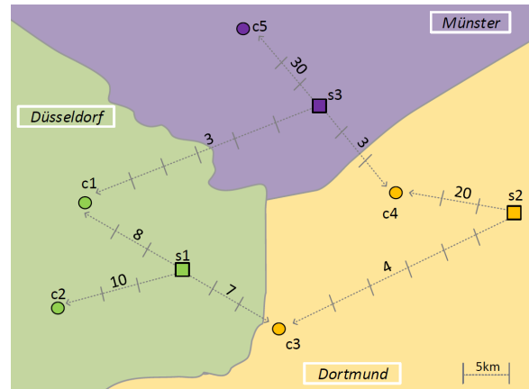
Fig. 5. Example map of Sales (instance) data
