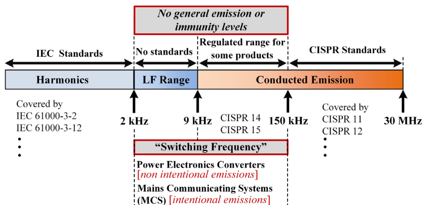
Figure 1 Harmonic and conducted EMI frequency ranges classified by IEC for distribution networks
