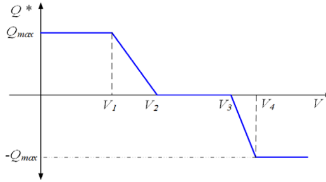
Fig.3- reactive power control of DG units
