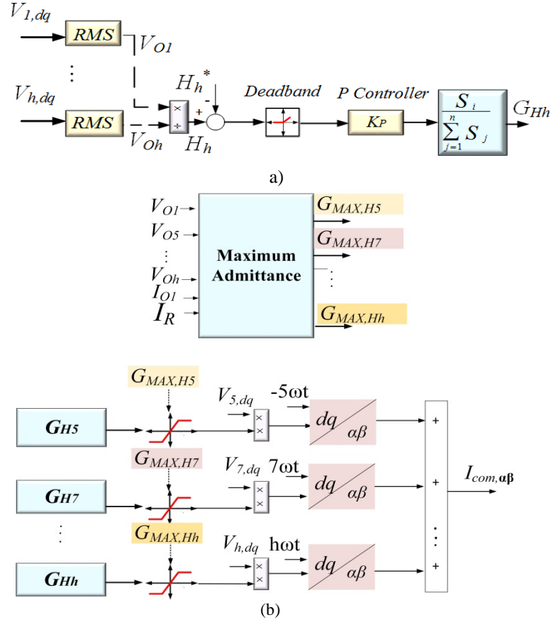
Fig. 5. Details of virtual admittance block of Fig 2; (a) G_{Hh} calculation block; (b) overall scheme
