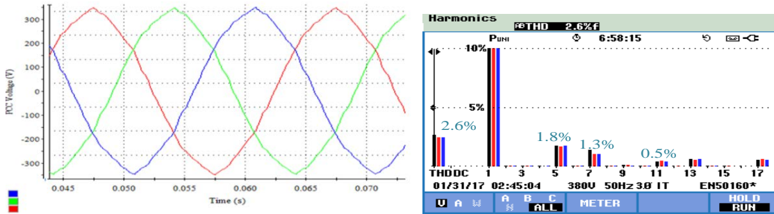
Fig. 13. PCC voltage before harmonic compensation in third scenario (Experimental results), a) voltage waveform, b) harmonic content
