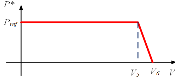
Fig. 4. Voltage rise mitigation by using power curtailment
