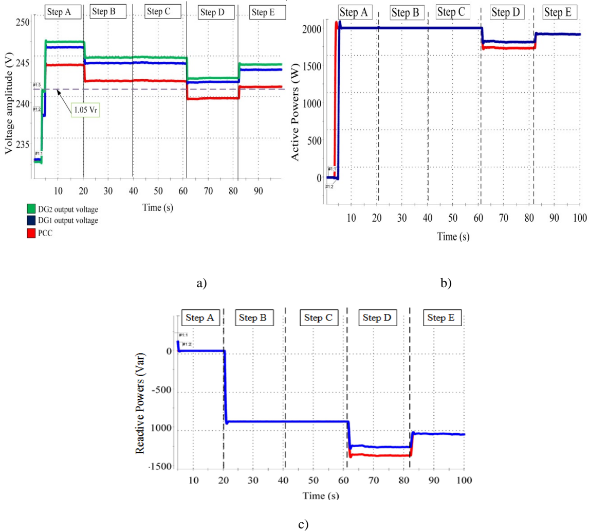
Fig. 12. Experimental results in second scenario with 233 V grid voltage, a) voltage amplitude, b) active power, c) reactive power
