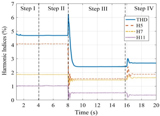
Fig. 8. Harmonic indices of PCC voltage in different steps of first scenario.
