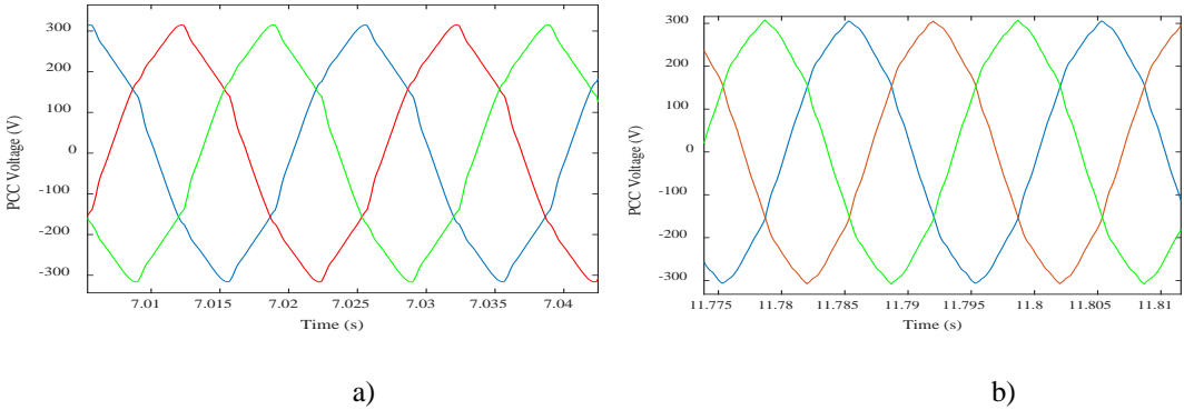
Fig. 9. PCC voltage in first scenario, a) before compensation (in Step II), b) after compensation (in Step III)
