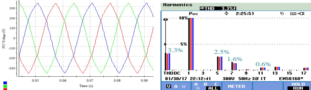
Fig. 14. PCC voltage, with communication system and 5ms delay in third scenario (Experimental results) a) voltage waveform, b) harmonic content
