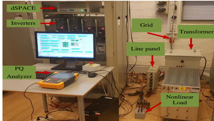
Fig. 10. Experimental setup of the grid tied inverters
