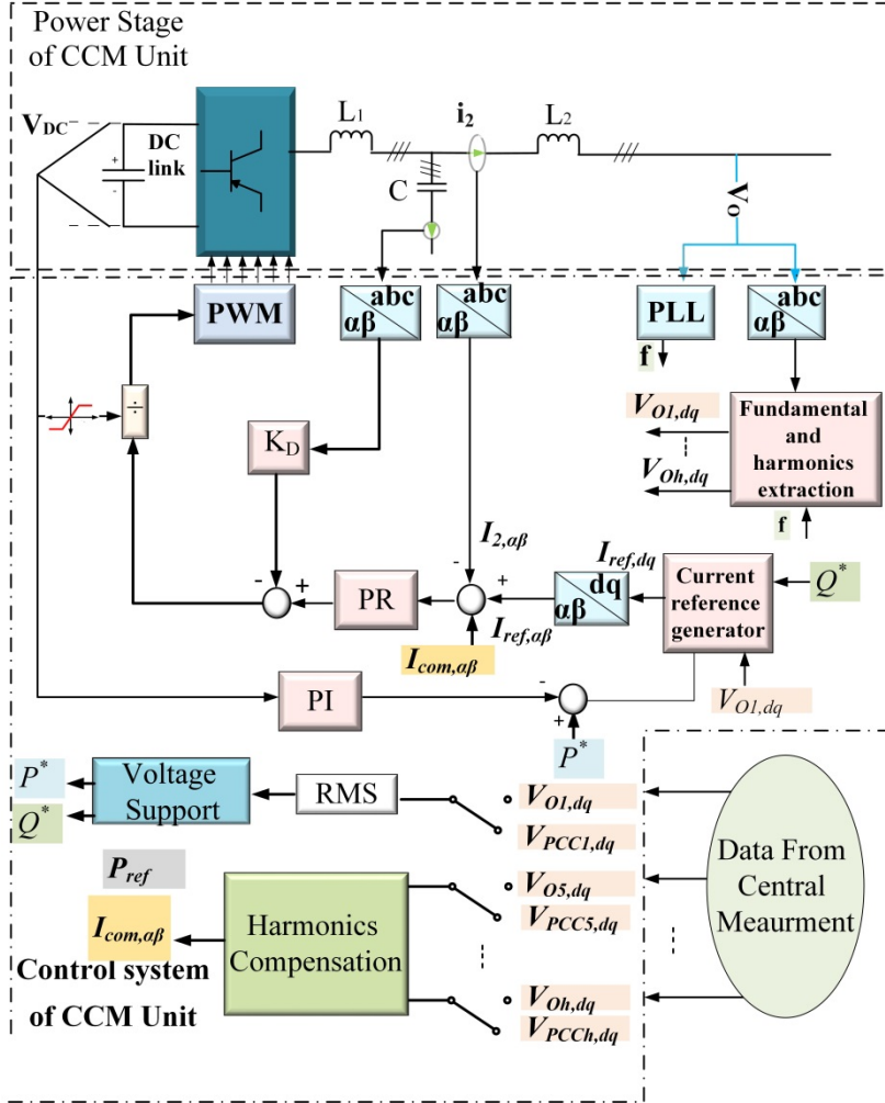
Fig. 2. Power and control stage of DG interfacing inverter
