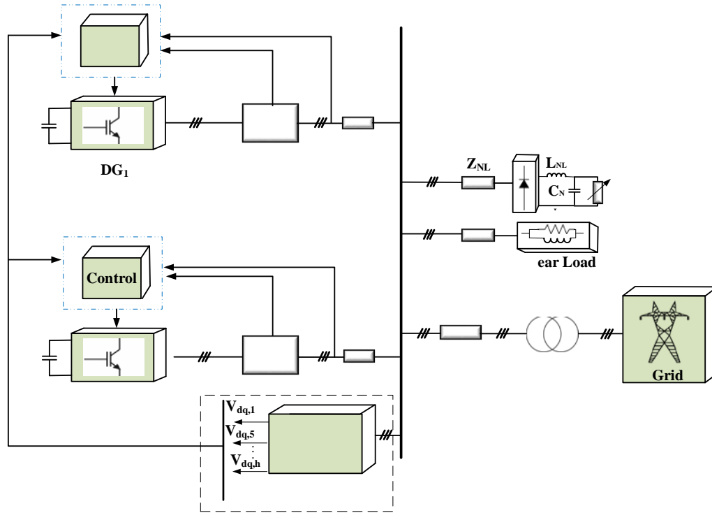
Fig. 1. General overview of the system
