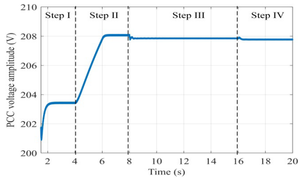
Fig. 7. Voltage amplitude in first scenario
