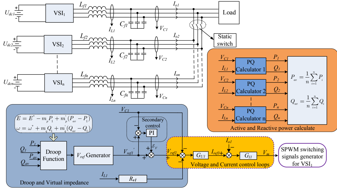
Fig. 2. The block diagram of the control structure with the modified droop control.
