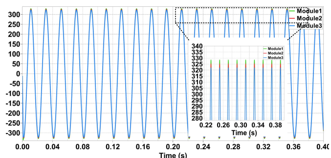
Fig. 18. The reference voltages of three modules under case3.
