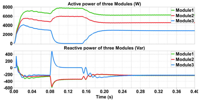
Fig. 21. Output power of three modules under case3 with conventional control.
