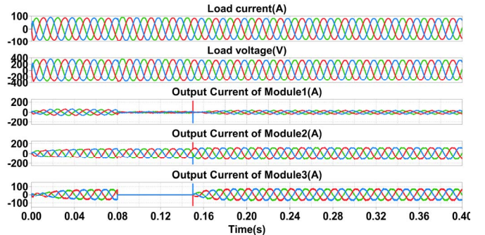
Fig. 12. Simulation results under case2 with the conventional control.
