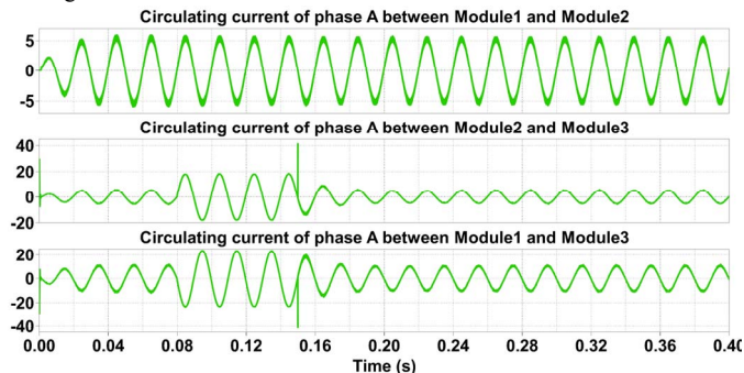
Fig. 20. Circulating currents among three modules under case3 with conventional control.
