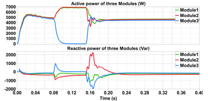
Fig. 11. Output power of three modules under case1 with proposed control.
