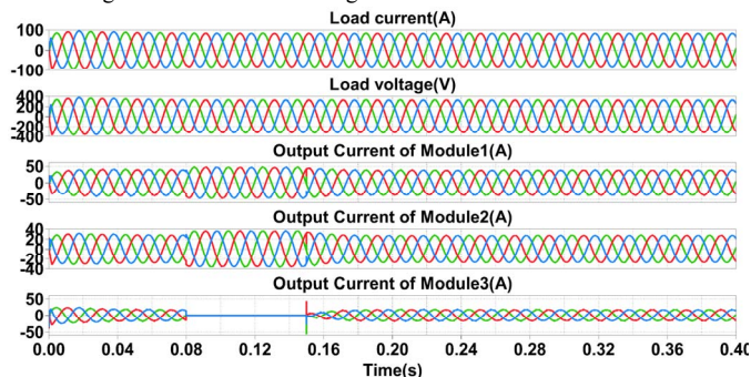
Fig. 19. Simulation results under case3 with the conventional control.
