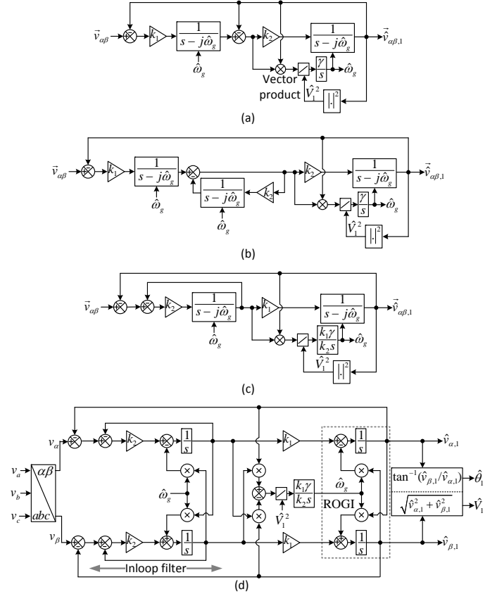
Fig. 19. (a) SOSF-FLL described with the complex signal flow graph, and (b) and (c) its alternative representations. (d) scaler realization of Fig. 19(c).
