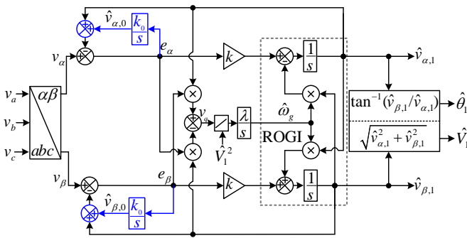
Fig. 3. An FLL with enhanced DC offset rejection capability.
