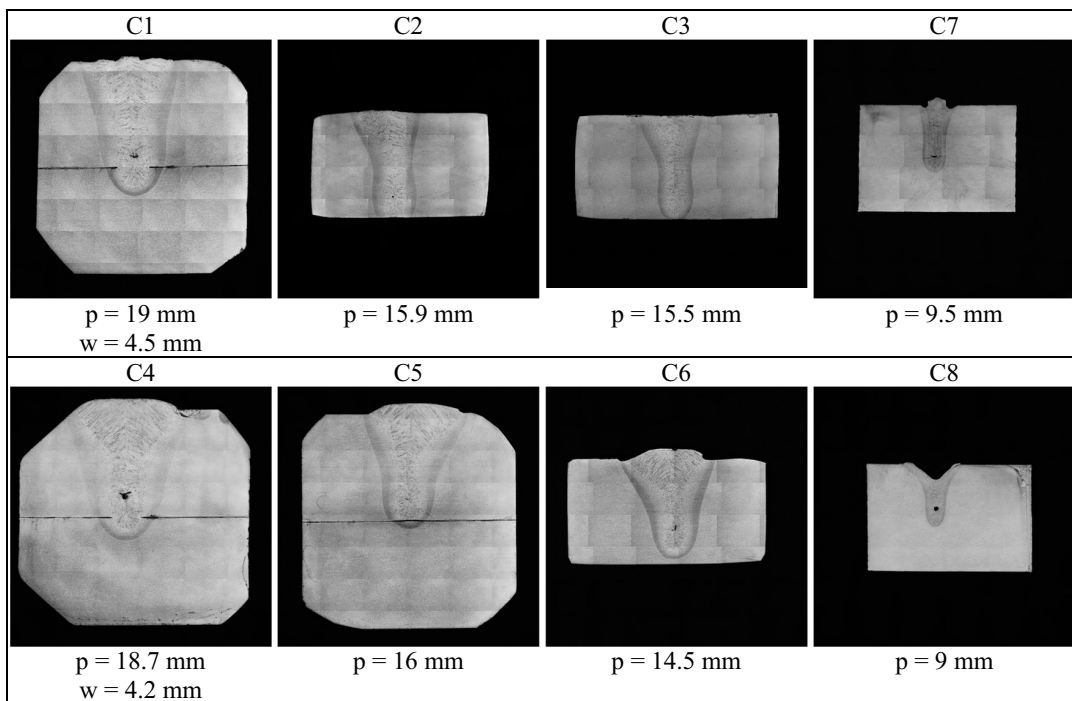
Fig. 6. Weld macro-sections of the lap joints and their corresponding penetration depths (p). The weld width (w) was measured at the joint interface for the penetration depths above 16 mm.
