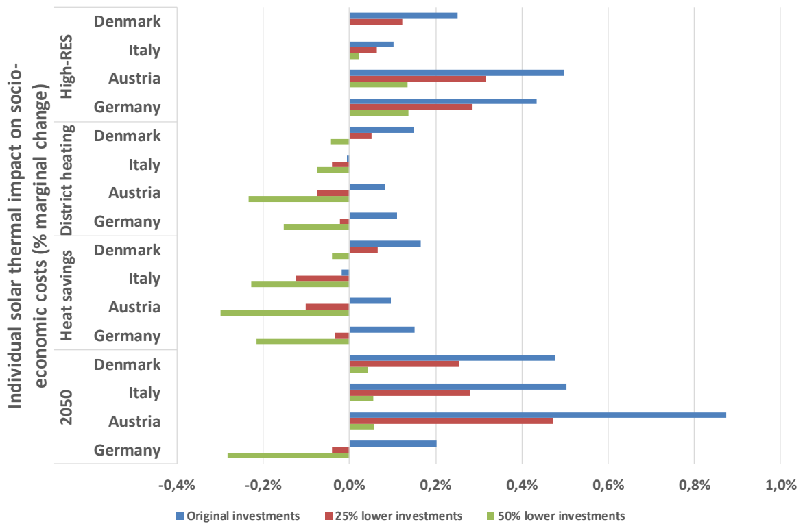
Figure 98: Marginal socio-economic cost changes for individual solar thermal potentials. The maximum potentials are installed in all the countries for three different solar thermal investment price levels; original as assumed in previous analyses with 2050 solar thermal prices, and with additional 25% and 50% lower investment prices.
