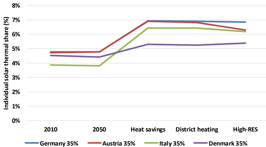
Figure 3: Solar thermal share potentials for individual heating in the four countries with a solar thermal penetration rate of 35%. The solar thermal share in the district heating areas is 6-10% of the total district heat production with a 35% solar penetration rate as shown in Figure 4. This indicates that the solar thermal share can be higher in district heating areas than in individually supplied areas and is caused by further options to store and share the heat between consumers and the larger flexibility through technologies such as CHP plants and heat pumps.
