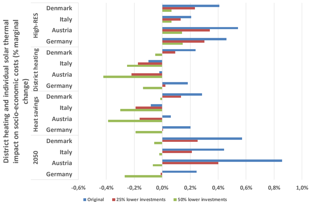
Figure 100: Marginal socio-economic cost changes for individual and district heating solar thermal potentials. The maximum potentials are installed in all the countries for three different solar thermal investment price levels; original as assumed in previous analyses with 2050 solar thermal prices, and with additional 25% and 50% lower investment prices.
