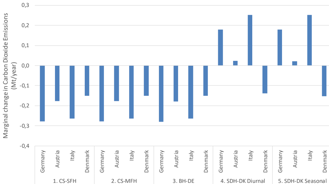
Figure 64: Marginal changes in CO 2 -emissions in the 2010 scenarios when installing 1 TWh of solar thermal.
