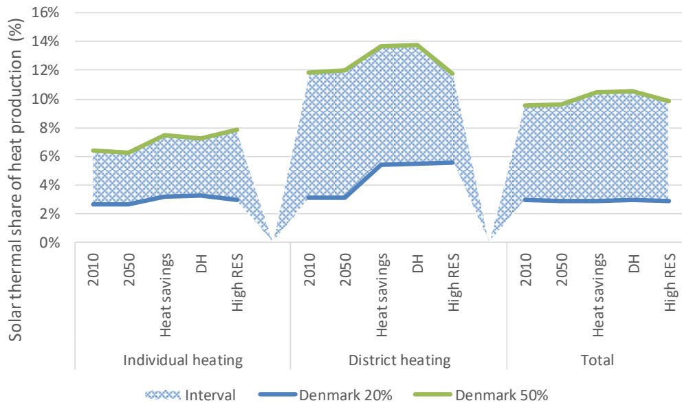
Figure 76: Danish solar thermal potential share of the heat production for individual heating and district heating under different conditions.
