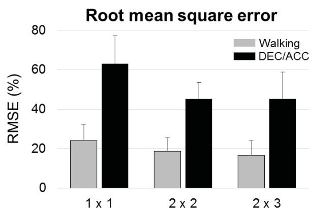
Figure 3 Relative root mean square error (RMSE) calculated between resultant speed extracted from an inertial and an optical motion capture system during walking (gray bars) and while decelerating, stopping and accelerating again (DEC/ACC, black bars).
