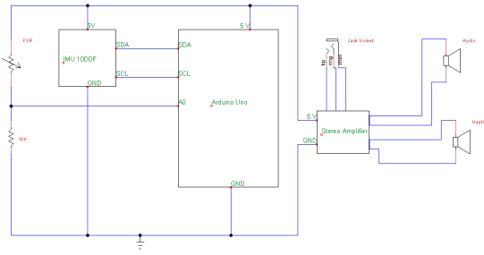
Figure 2: Schematic of bEADS circuitry
