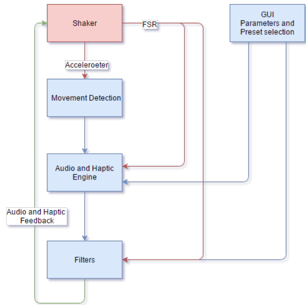
Figure 3: Coarse overview of the bEADS system
