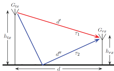
Fig. 1: Simplification with the 2 Ray model.
