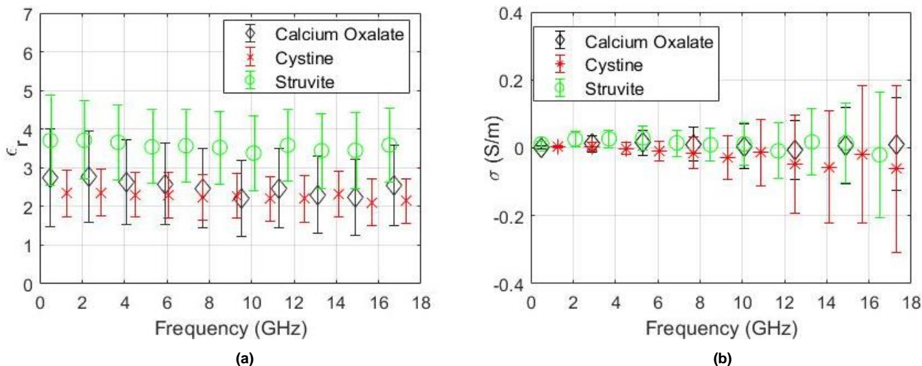
Figure 3. Median dielectric property measurements of calcium oxalate, cystine, and struvite obtained from patients; (a) median relative permittivity comparison (b) median conductivity comparison.
