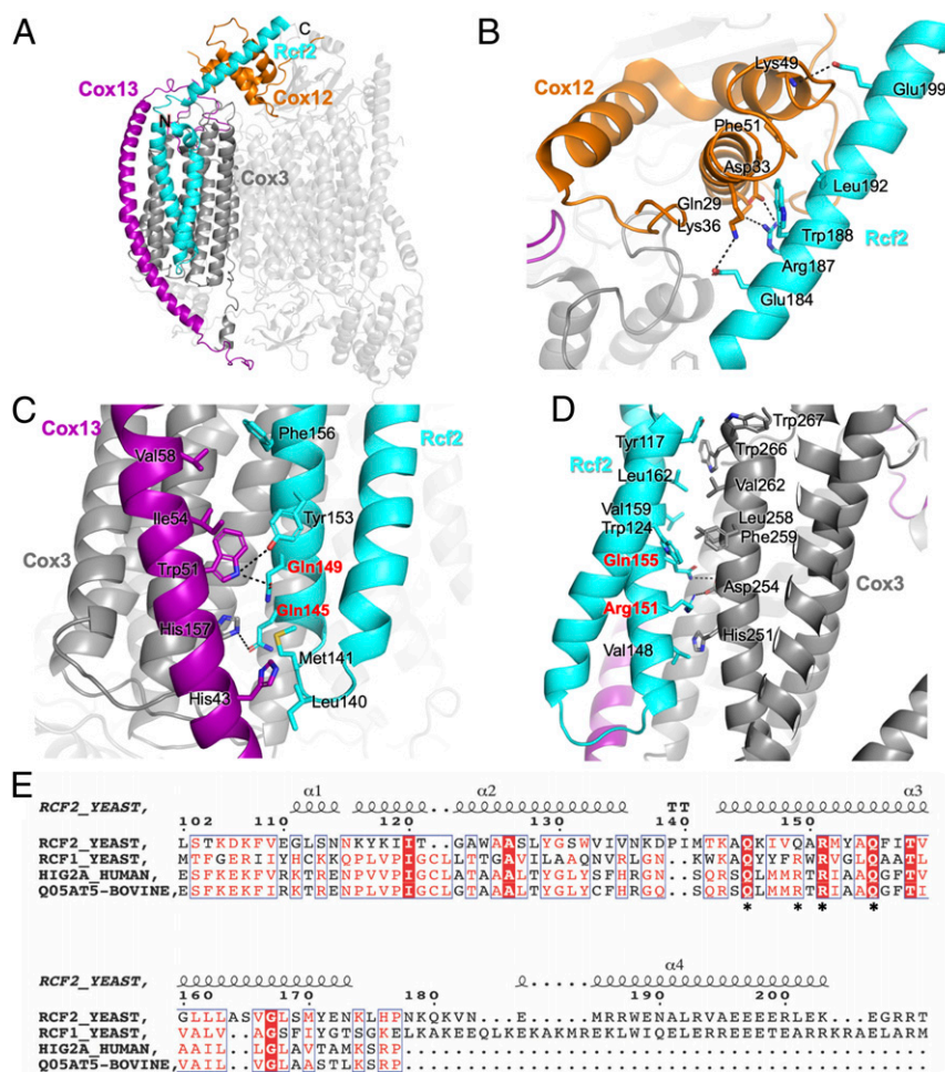
Fig. 4. Rcf2 is revealed in the \Delta rox1 III 2 -IV 5B 1 SC structure. (A) Structure of CIV in the \Delta rox1 III 2 -IV 5B 1 SC with Rcf2 (cyan), Cox3 (dark gray), Cox12 (orange), and Cox13 (purple) highlighted. (B) Interactions between the C-terminal helix of Rcf2 and Cox12 in the IMS. Residues that form interactions are labeled. (C) Interactions within the IMM between Rcf2 and Cox3 and Cox13. (D) Interactions within the IMM between Rcf2 and Cox3. Residues of the conserved Q(R/Q)RQ motif of Hig1 type 2 proteins are highlighted in red. (E) Sequence alignment of yeast Rcf2 (Uniprot: P53721), Rcf1 (Q03713), human Hig2a (Q9BW72), and bovine Hig2a (Q05AT5). The numbers above the sequences correspond to the Rcf2 sequence. The alignment shows only the fraction of the determined Rcf2 structure, highlighting the HIG1 domain (residues 110 to 177) and the conserved Q(R/Q)RQ motif (stars underneath the sequences). The secondary structure elements for Rcf2 are displayed above the sequence. The image was generated in ESPript (53).
