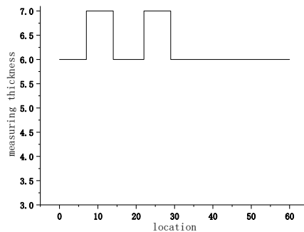
Fig. 1. Determination of aluminum layer thickness in anchor grooves of steel with tension line
