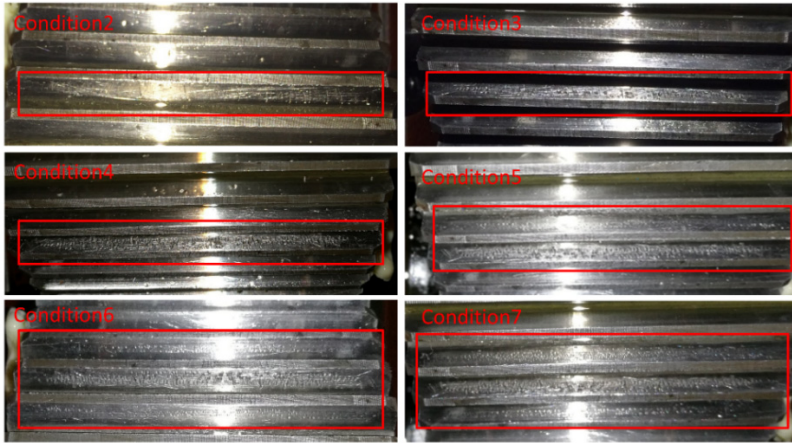
Fig. 3. Pitting degree of driven gears
