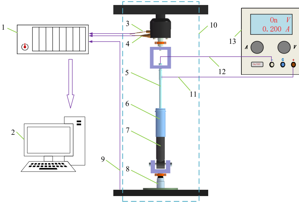
Fig. 1. Experiment system for testing friction force of MR damper featuring three bypass holes:
