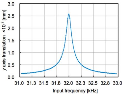
Fig. 5. Frequency response analysis
