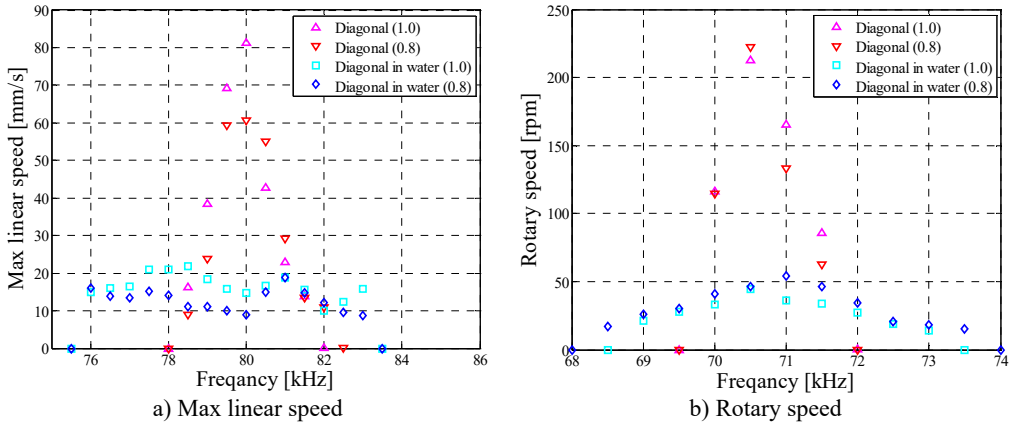
Fig. 7. Frequency characteristics in water (Polyvinyl resin)
