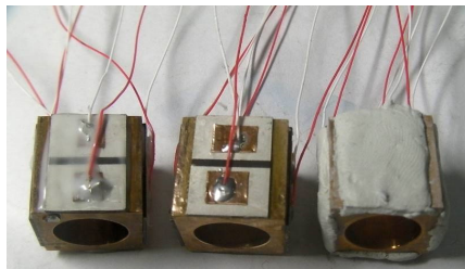
Fig. 5. TR motors with Silicone rubber, Poly vinyl resin and Epoxy putty from the left
