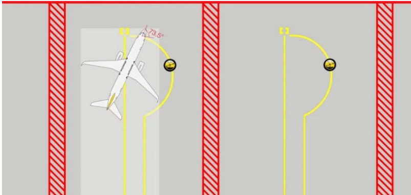
Fig. 4. Turning on the spot with a NW steering angle of 73.5°
