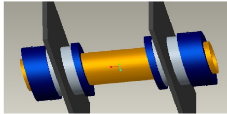
Fig. 2. Three-dimensional model of pipe penetration piece
