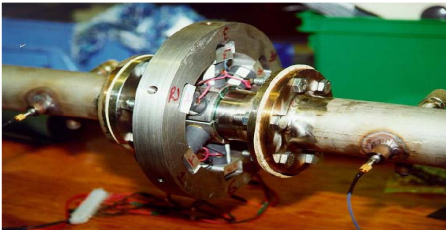
Fig. 1. Real figure non-submerged device
