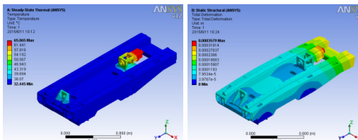
Fig. 7. The temperature field and thermal-deformation of 32 ^\circ\text{C} without TCR
