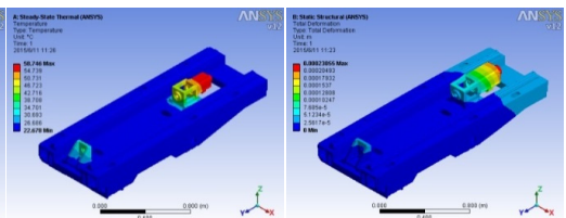
Fig. 6. The temperature field and thermal-deformation of 20 ^\circ\text{C} with TCR
