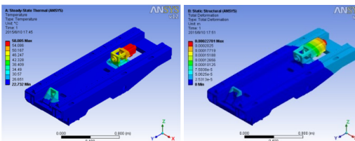
Fig. 5. The temperature field and thermal-deformation of 20 ^\circ\text{C} without TCR
