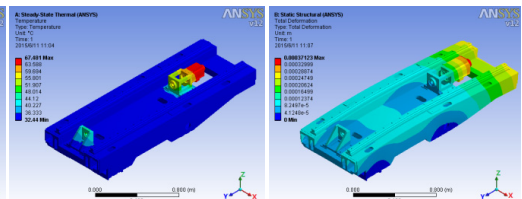
Fig. 8. The temperature field and thermal-deformation of 32 ^\circ\text{C} with TCR
