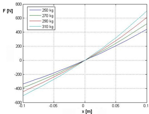
Fig. 6. Dynamic force vs. displacement characteristics for different static loads in a hydropneumatic strut (Citroën BX front strut)
