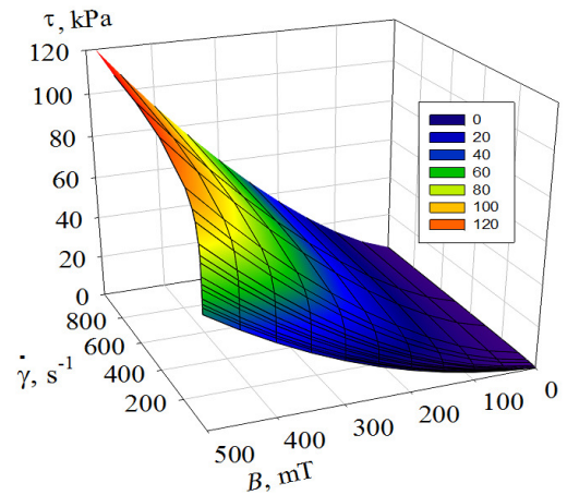
Figure 4. The dependence of shear stress \tau of the MR fluid on shear rate \dot{\gamma} and different values of magnetic flux density B by the model (8).
