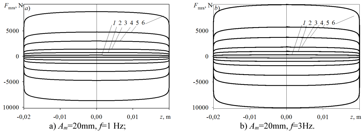
Figure 5. The dependence of MR shock-absorber force from rod displacement z at different values of magnetic flux density B : 1 – B=0 mT; 2 – 50; 3 – 100; 4 – 200; 5 – 300; 6 – 500.
