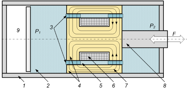
Figure 1. The scheme of the MR shock-absorber: 1 – the cylinder; 2 – a MR fluid without the magnetic field; 3 – a MR fluid in the magnetic field; 4 – the piston; 5 – the annular channel; 6 – the solenoid; 7 – the magnetic field lines; 8 – the rod; 9 – the pneumatic camera with a gas.
