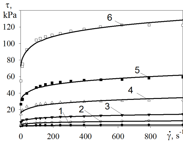
Figure 3. The dependence of shear stress \tau of the MR fluid on shear rate \dot{\gamma} at different values of magnetic flux density B : 1 – B=0\text{mT} ; 2 – 50; 3 – 100; 4 – 200; 5 – 300; 6 – 500. Points – experiment; lines – the model (8).
