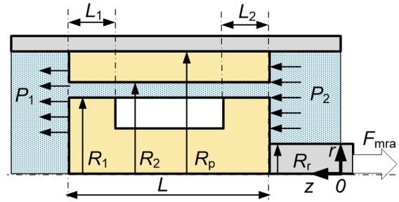
Figure 2. The geometry of the annular channel of the piston of the controlled shock-absorber with a MR fluid in the cylindrical coordinate system.
