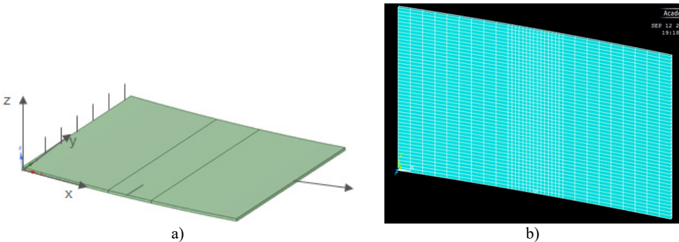
Fig. 3. Geometry of curved plate with crack (a), FE model of curved plate with crack (b)
