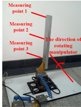
Fig. 1. The manipulator
