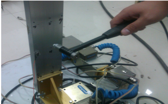
Fig. 5. Hammer experiment
