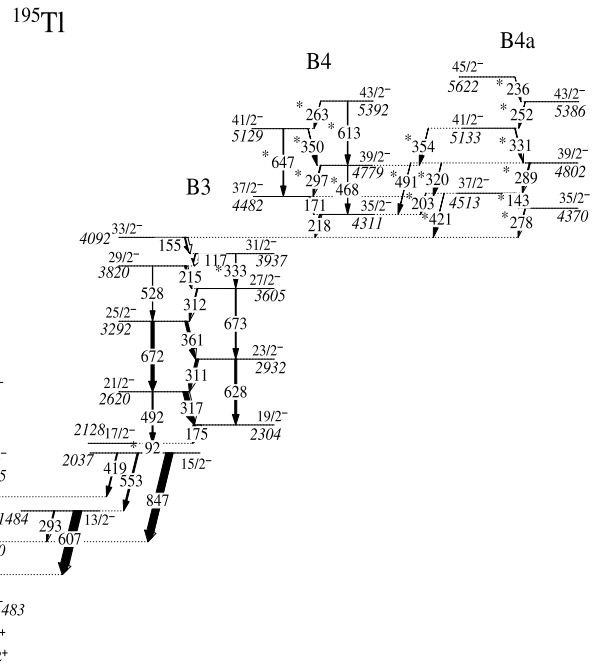
Fig. 3. Partial level scheme of ^{195}\text{Tl} proposed from the present work. The newly observed transitions are marked by asterisks (*). The width of the transitions are proportional to their intensity.
