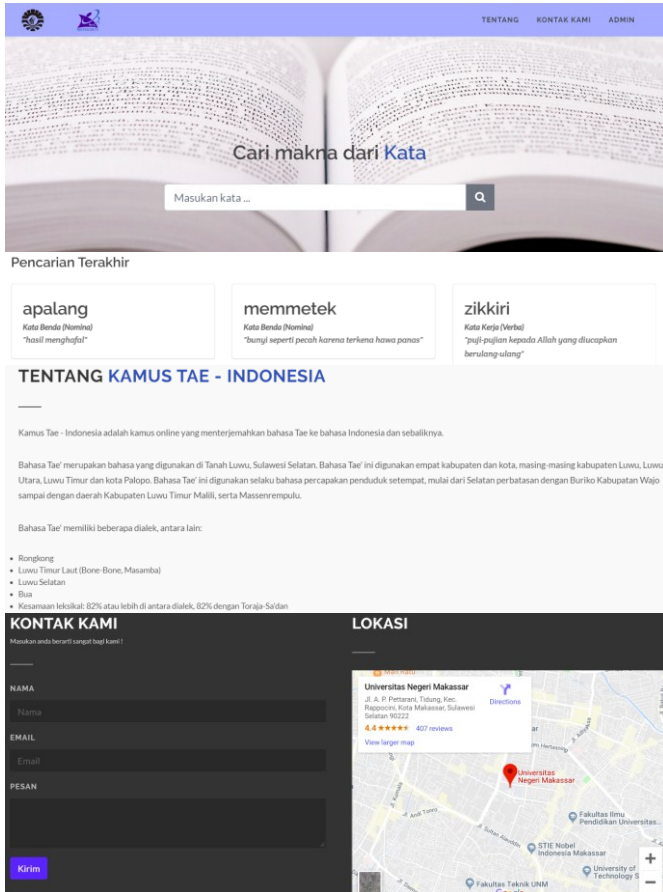
Gambar 2 Front End
