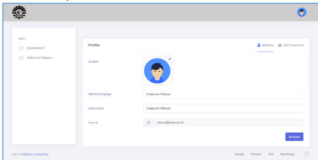
Gambar 10 Profile
