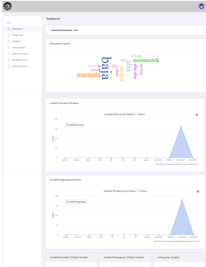
Gambar 19 Dashboard Admin
