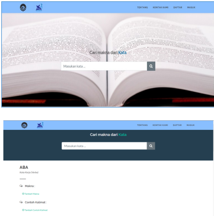
Gambar 3 Detail Kata
