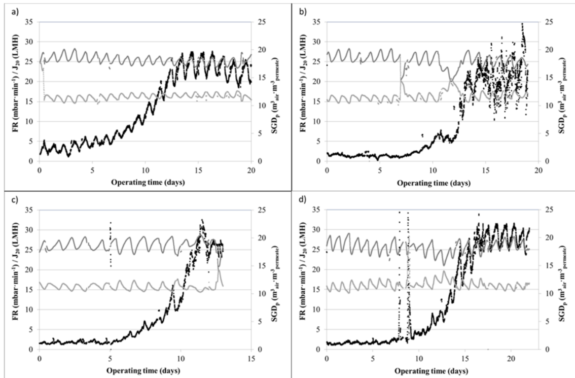
Figure 8. Membrane filtration performance at the pilot plant. Fouling rate (—) ( \text{mbar}\cdot\text{min}^{-1} ), J_{20} (—) (LMH) and \text{SGD}_p (—) ( \text{m}^3_{\text{air}}\cdot\text{m}^{-3}_{\text{permeate}} ) for: a) HRT3.5; b) HRT2; c) HRT1.5; d) HRT1
