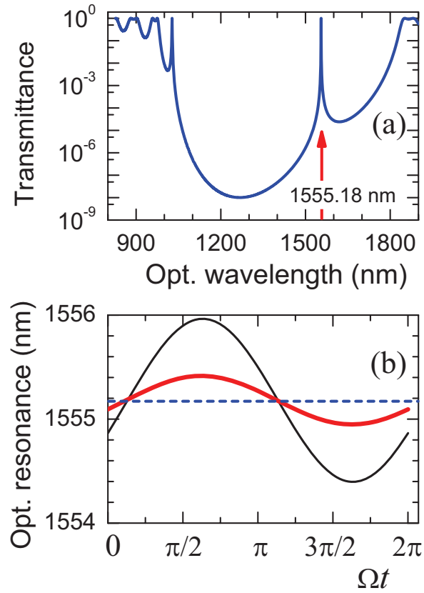
Figure 2: (a) Optical transmission spectrum of the phoxonic crystal under study, at normal incidence, without the AO interaction. The optical resonance appears at 1555.18 nm. (b) Oscillatory behavior of the optical resonance as a function of time for the attenuated acoustic excitation at resonance (thick line) compared to the lossless acoustic excitation (thin line). The input displacement level is u_0 = 0.1 nm in both cases.
