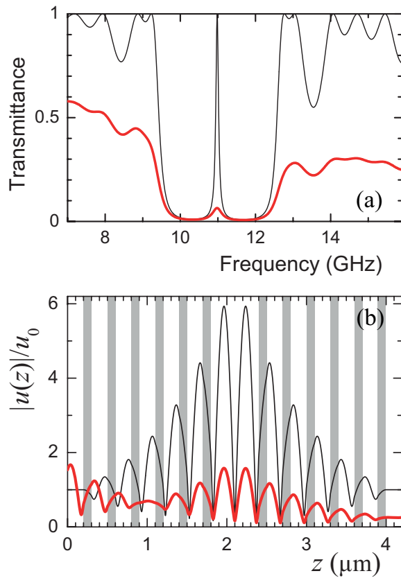
Figure 1: (a) Phononic transmission spectrum of a compressional acoustic wave normally incident on the phoxonic crystal under consideration without (thin line) and with (thick line) losses. (b) Displacement amplitude profile, normalized to the input displacement level u_0 , at the acoustic resonance without losses (thin line) and with hypersonic attenuation taken into account (thick line). White and gray stripes in the background show the regions of \text{SiO}_2 and Si, respectively.
