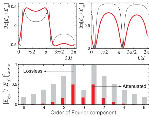
Figure 3: Optical reflection through the given phoxonic structure under a continuous acoustic excitation of input level u_0 = 0.1 nm, for normally incident light at the resonance wavelength with electric field amplitude E_{inc} . Time variation of the perturbed reflected optical field (upper diagrams) and intensities associated with the corresponding Fourier components (lower diagram). The perturbation refers to the AO interaction with the acoustic excitation at the resonance frequency of 10.86 GHz with hypersonic attenuation. For comparison, the corresponding lossless acoustic excitation graphs are shown as thin lines in the upper diagram and as grey background bars in the lower one. The Fourier components on the lower panel are normalized with respect to the first order component with a resonant acoustic excitation without losses.
