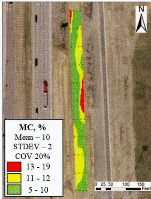
Figure G.17 – Spatial Distribution of Moisture Content of Flexible Base Layer.
