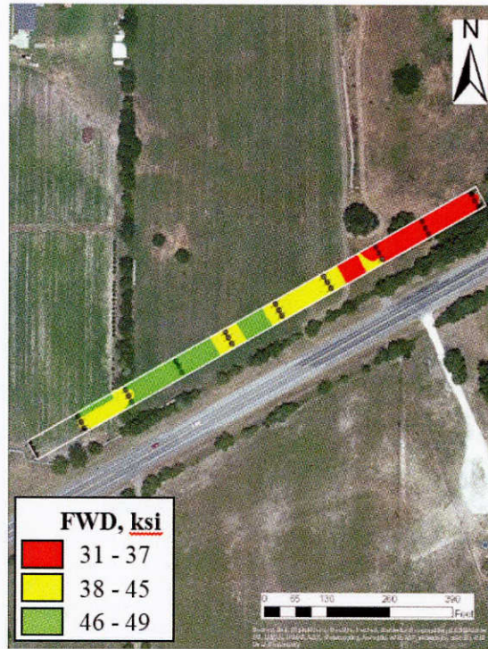
Figure F.11 - Spatial Variation of FWD Modulus on Compacted CTB Layer.
