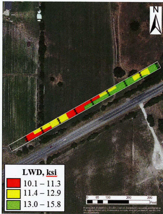
Figure F.14 - Spatial Variation of LWD Modulus on Compacted FB Layer.
