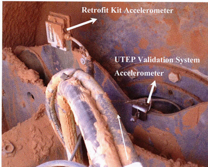
Figure D.2 - Mounted Accelerometers from IC Retrofit Kit and UTEP Validation System.
