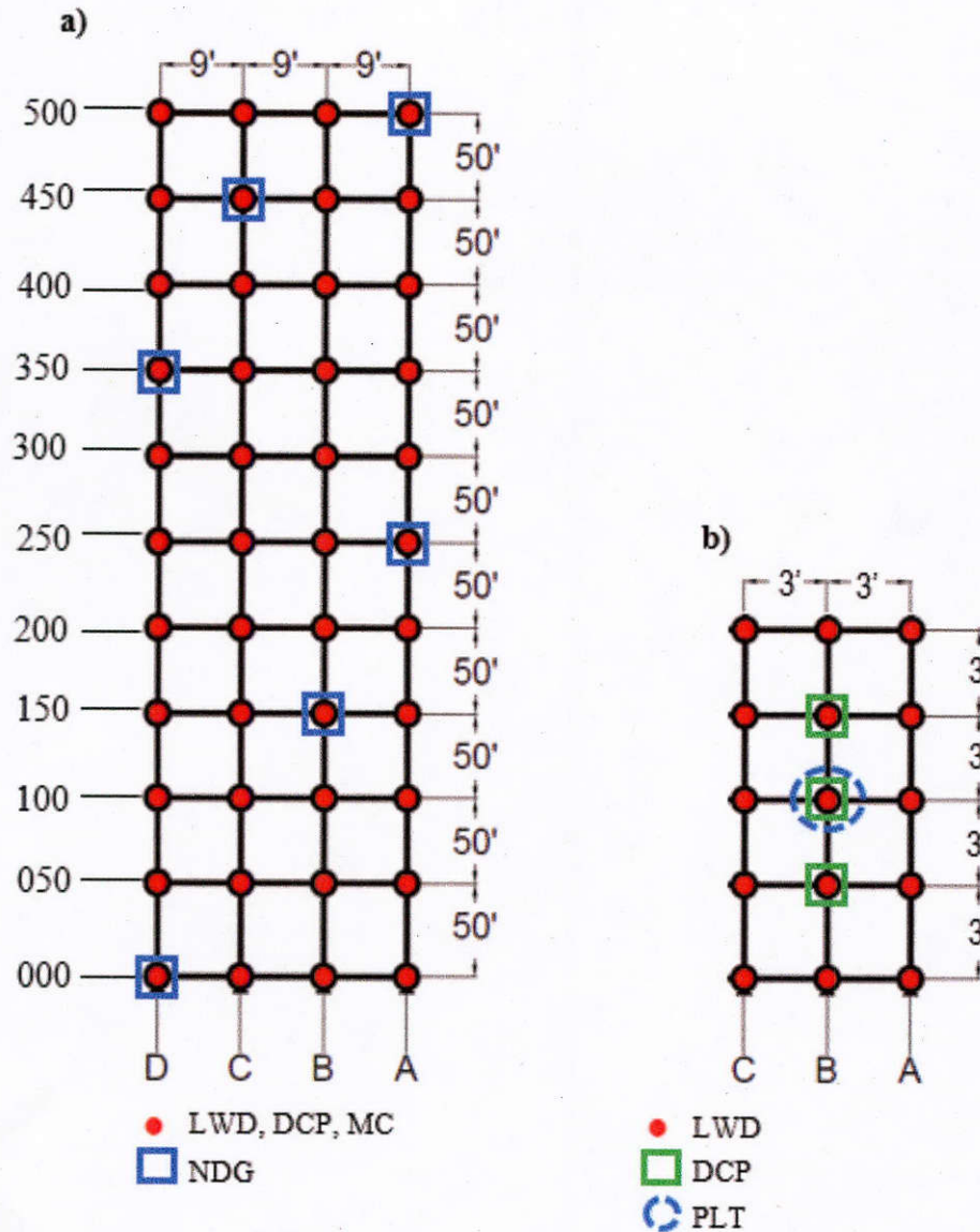
Figure G.2 a) Schematic of the Typical Test Section and Location of Spot Tests and b) Diagram of the Testing Area around the PLT Locations.
