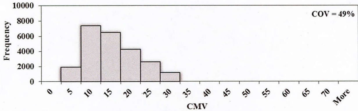
Figure F.4 - Distribution of CMV Data during Pre-Mapping of Existing Subgrade Layer.
