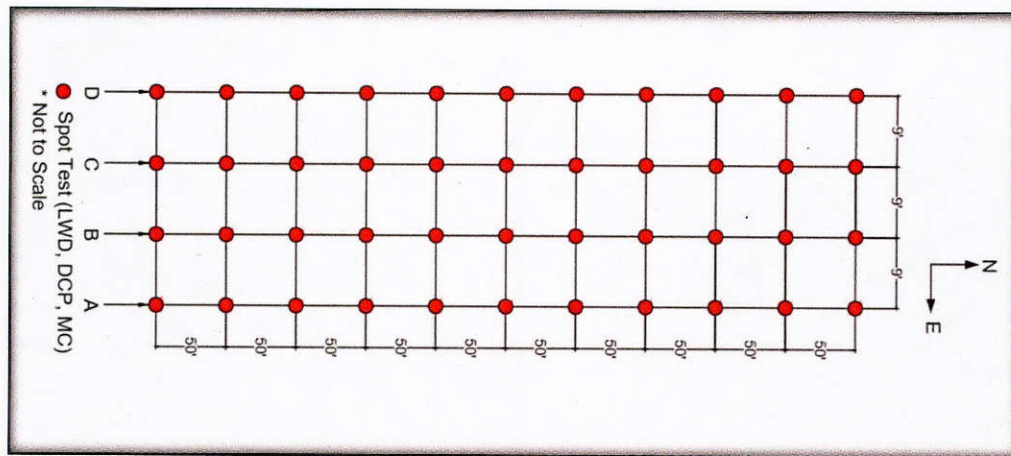
Figure 3.1 – Schematic of a Typical Test Section and Locations of Spot Tests.
