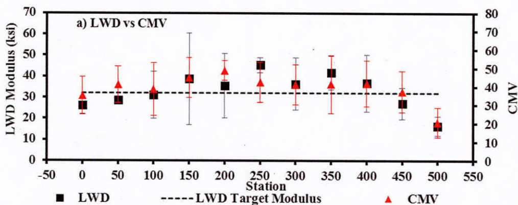
Figure 3.5 – Relationship Between Averaged LWD Modulus vs. ICMV.
