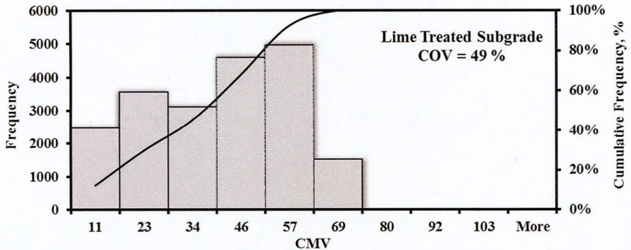
Figure G.5 - Distribution of CMV Data Collected by IC Roller during Proof-Rolling of LTS Layer.
