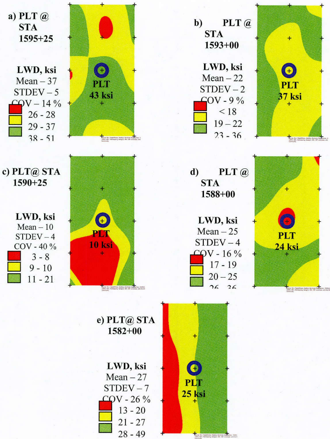
Figure G.11 – Spatial Distribution of LWD at Different PLT locations.
