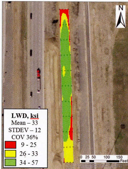
Figure G.6 – Spatial Distribution of LWD Modulus on LTS Layer.
