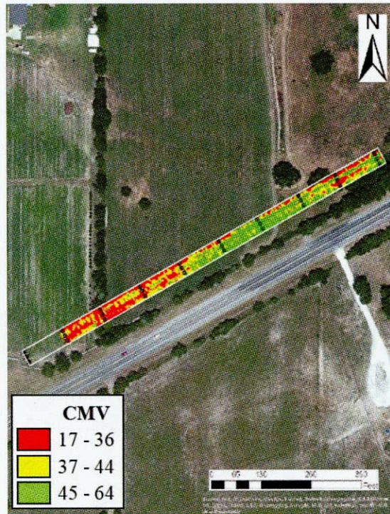
Figure F.12 - Spatial Distribution of CMV Data from IC Retrofit System during Mapping of Compacted FB Layer.
