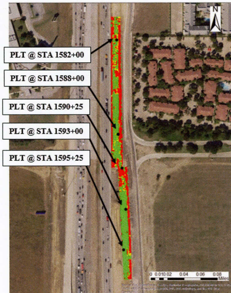
- Figure G.3 Aerial View of the PLT Locations.
