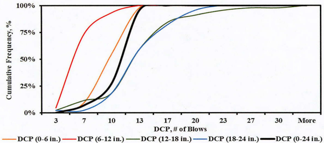
Figure G.8 – Cumulative Distribution of Number of DCP Blows in LTS Layer.
