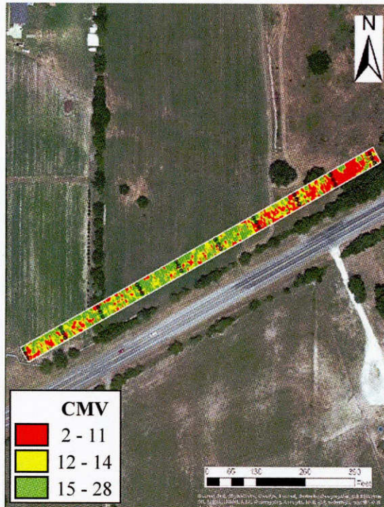
Figure F.2 - Spatial Distribution of CMV Data Collected by IC Retrofit System during Pre-Mapping of Existing Subgrade Layer.
