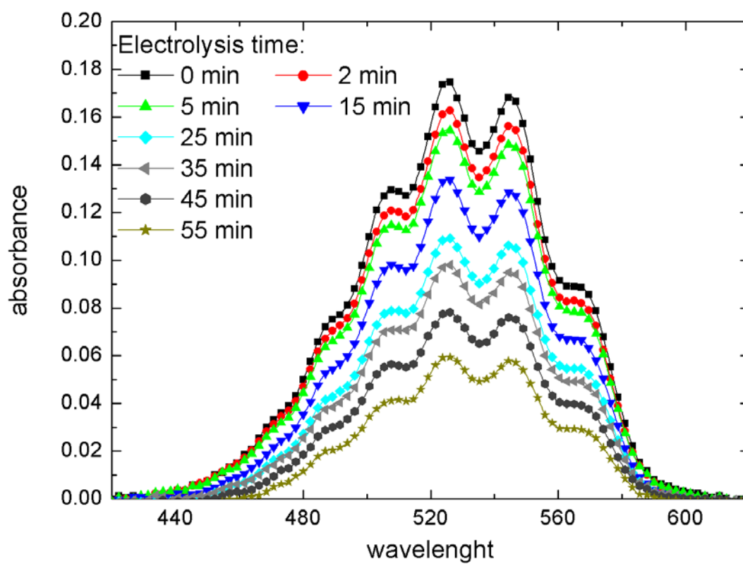
Fig. 8 Evolution of the absorbance spectra of \text{KMnO}_4 aqueous solutions during continuous AIROF electrode scanning in \text{N}_2 -saturated 0.5 \text{ M H}_2\text{SO}_4 from 1.5 to 2 V at 100 \text{ mV/s}
