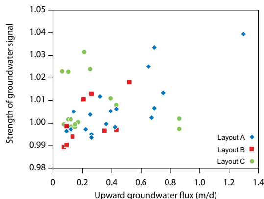
Figure 5. Correlation of the strength of the groundwater signal as recorded by DTS with upward groundwater fluxes estimated from VTPs. Measurements from each layout are separated by colour.
