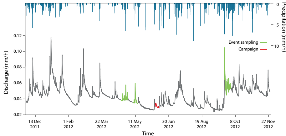
Figure 2. Precipitation and discharge during 2011–2012. Upper part: hourly precipitation measured 6 km northwest of station 4. Lower part: the measured discharge at the catchment outlet (station 4).
