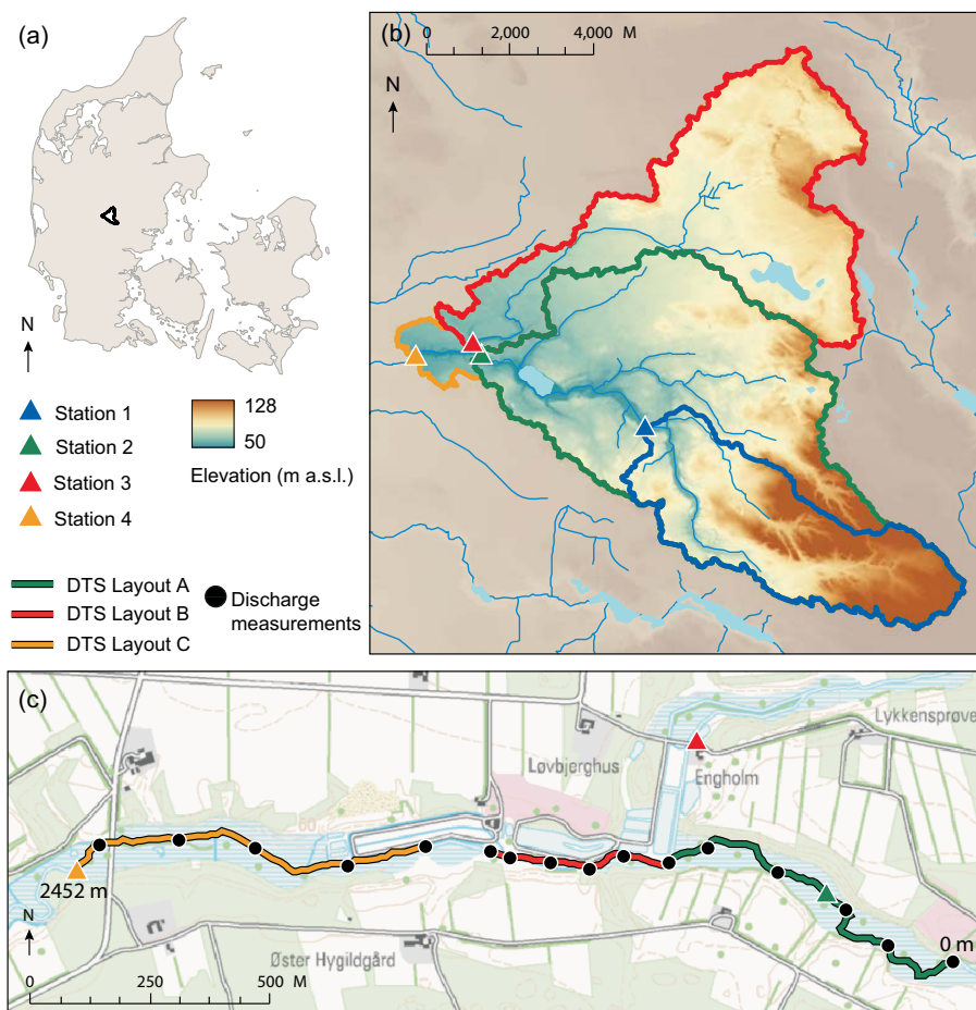
Figure 1. Map of the study area and sampling sites. (a) Map of the study area in Jutland, Denmark, showing the Skjern River catchment and sampling sites. At this site, the stream flows from east to west. (b) Locations of the stations of event samplings and their corresponding catchments. (c) The campaign measurements conducted between station 2 and station 4.
