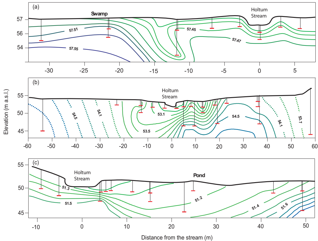
Figure 3. Manually interpolated cross-sectional contour maps of hydraulic heads. (a) Cross section at station 1 based on data from February 2013. (b) Cross section at station 2 based on data from June 2013. (c) Cross section at station 4 based on data from March 2012. The horizontal red lines represent the screen depth of the piezometers where hydraulic heads were measured. Dashed isopotential lines indicate areas with sparse data coverage.
