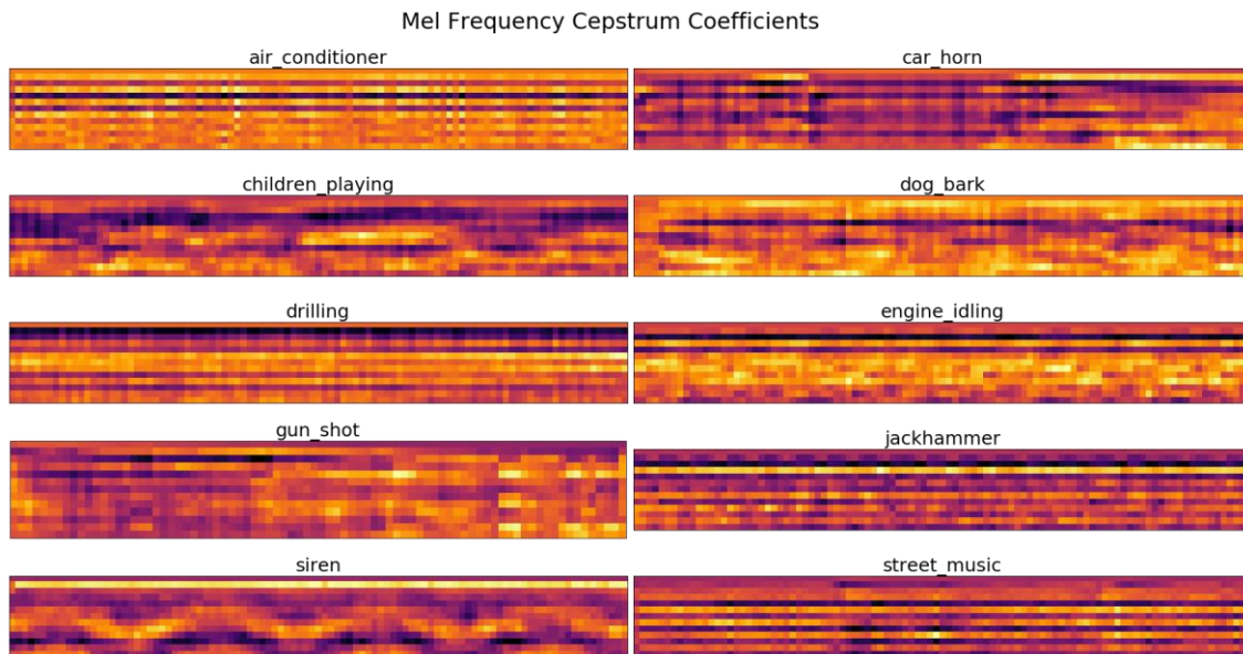
Figure 3.7 - Mel-Frequency Cepstrum Coefficients for one second of the 10 analyzed classes
