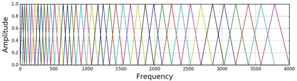
Figure 2.9 - Filter bank with 40 filters on a Mel-Scale [27]
