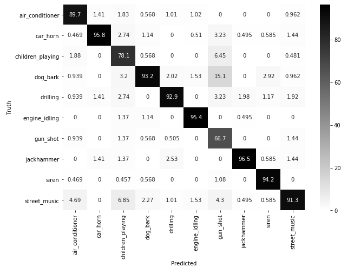
Figure 4.4 - Confusion matrices for the NN model using a) 10, b) 13, c) 20 and d) 40 MFCCs
