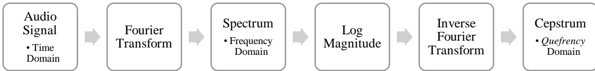
Figure 2.7 - Transformation from Audio Signal into Cepstrum (Adapted from [21])
