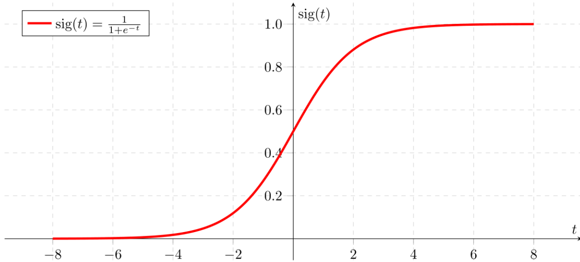
Figure 2.12 - Sigmoid function [35]
