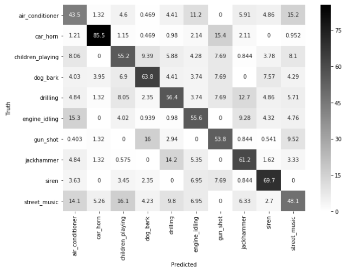
Figure 4.1 - Confusion matrices for the LR model using a) 10, b) 13, c) 20 and d) 40 MFCCs
