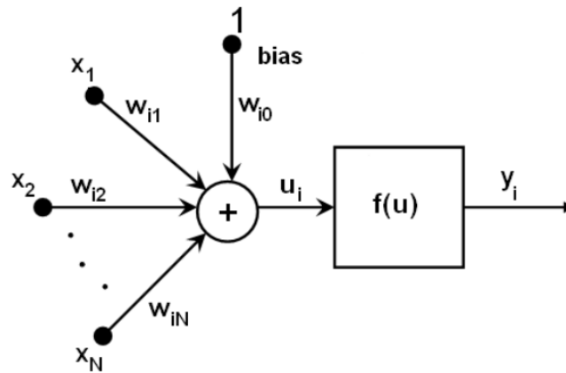
Figure 2.18 - Shape and function of a neuron [42]
