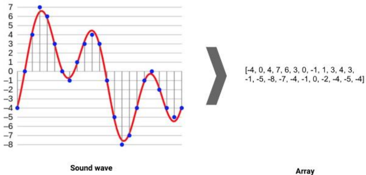
Figure 2.3 - A sound wave, in red, represented digitally, in blue (after sampling and 4-bit quantization), with the resulting array shown on the right [19]
