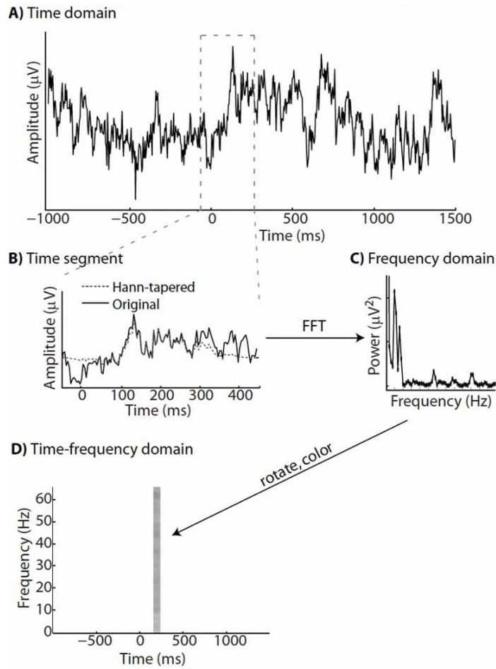
Figure 2.5 - The process of obtaining a spectrogram [22]
