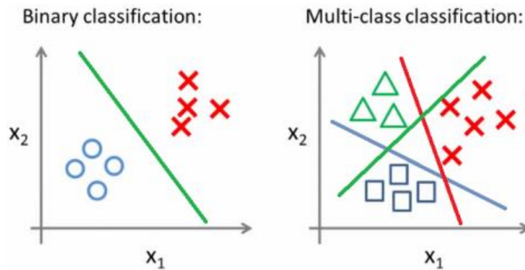
Figure 2.13 - Binary classification and multi-class classification [36]
