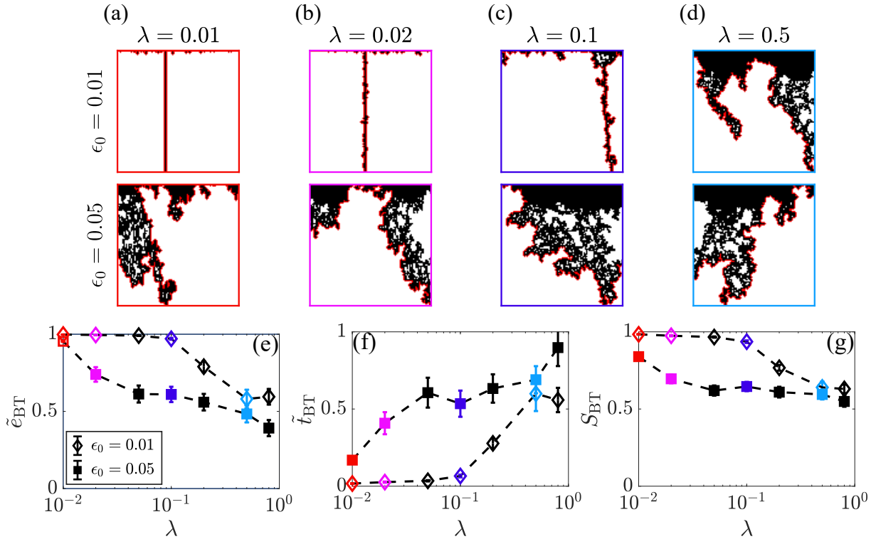
Figure 5: Low pore-size disorder \lambda increases the sensitivity of drying patterns to matrix deformation, resulting in preferential drying patterns (a–d) which maintains liquid connectivity to the open surface (top of the sample). This provides higher drying rates and shorter time at breakthrough (e–f), which is achieved at higher saturation (g). Lower \epsilon_0 increase the magnitude of particle displacement, thus maintaining the preferential drying behavior for higher \lambda . Symbols and error bars represent mean values and standard error from 20 realizations for each \lambda and \epsilon_0 . Colors of symbols match the boxes in (a)–(d).
