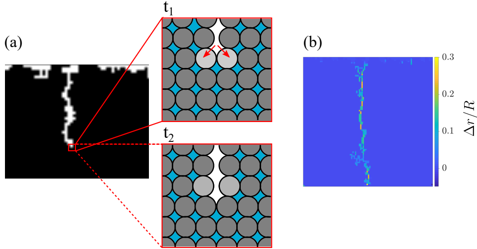
Figure 3: Preferential drying is associated with matrix deformation. The air finger in panel (a) is the consequence of progressive pore opening due to pressure imbalance (capillary pressure) acting on the particles at the finger tip. The insets show the particle positions (gray circles), before ( t_1 ) and after ( t_2 ) a particular pore invasion event, featuring the enlargement of the throat formed between the particle pair (highlighted in light gray) at the finger tip due to the pressure imbalance pushing the particles apart. Red arrows indicate the resultant pressure force acting on the particles, increasing the throat aperture and facilitating the next pore invasion at the finger tip, unless a larger throat is already accessible elsewhere. Air and liquid filled pores appear in white and blue, respectively. Panel (b) shows the change in the throat apertures, \Delta r , rescaled by the particle radius R (for simplicity only the vertical throats are plotted). If this deformation-assisted mechanism is dominant, the macroscopic drying pattern follow the path of the modified throat apertures, making it highly preferential, leaving most of the liquid behind at breakthrough.
