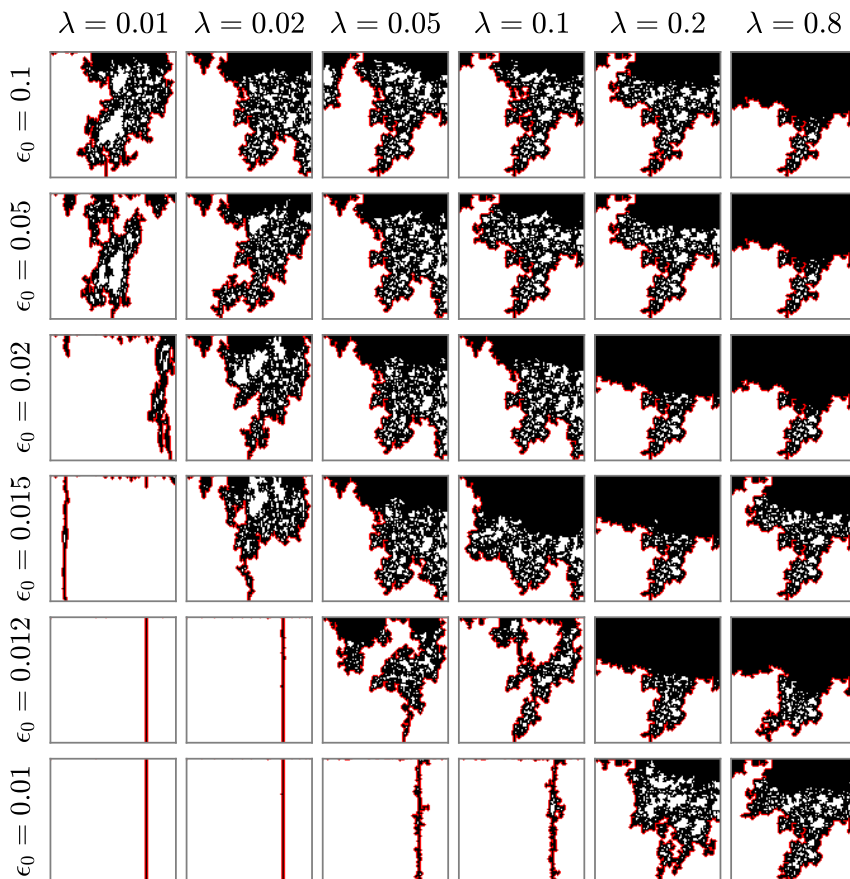
Figure 2: Drying patterns at breakthrough, demonstrating that lowering the initial disorder in throat sizes \lambda and the initial confinement \epsilon_0 promotes preferential drying patterns through matrix deformation, with thinner fingers of air that reach breakthrough while most of the medium is still wet. Black and white represent air- and liquid-filled pores, respectively; red line indicates the drying front. A single sample was used for all simulations in this diagram; that is, we used the exact same spatial distribution of throat sizes r (when varying \epsilon_0 ), and the same relative magnitudes of r (when varying \lambda ).
