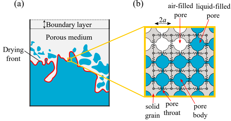
Figure 1: (a) Model schematics. The porous medium is open at one of its faces, where a vapor concentration gradient drives evaporation from the air-liquid interface, and out to the atmosphere through a diffusive boundary layer. As evaporation reduces liquid pressure, air invades into liquid-filled pores. Some of the liquid becomes disconnected and forms isolated clusters. The drying front (in red) represents the most advancing part of the interface. (b) We model evaporation and capillary invasion via a pore network model, which we couple with a block-spring model that captures the effect of capillary pressures on matrix deformation. Pore bodies represent the space between solid particles placed on a square lattice (with spacing of 2a ), and are interconnected by throats. Solid particles are illustrated here as dented blocks, a 2-D illustration that emphasizes that our model considers a network of contact forces between particles (represented by springs), while allowing fluid connectivity between the pores. Displacement of solid particles modifies the pore throats, impacting their capillary thresholds.
