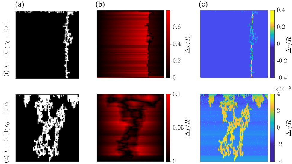
Figure 7: Different mechanisms underlie deformation-assisted preferential drying when the deformation is induced by lowering confinement and lowering disorder: (i) Low initial confinement (top row, \epsilon_0 = 0.01 ) leads to large particle displacements and significant changes in throat apertures, while (ii) low disorder (bottom row, \lambda = 0.01 ) enhances the impact of small displacements. In both cases, the drying patterns at breakthrough are preferential (a). (b) The magnitude of horizontal particle displacement |\Delta x/R| is significantly larger for low \epsilon_0 than for low \lambda , and centered around the invading air finger (b). Consequently, changes in vertical throat apertures \Delta r/R are more pronounced for low \epsilon_0 . We note that at low disorder, even small aperture changes impact the drying pattern, as evident from the equivalence of the pattern and deformations (panels a and c in bottom row). This is highlighted by the different scale in which the deformations are presented (panels b and c).
