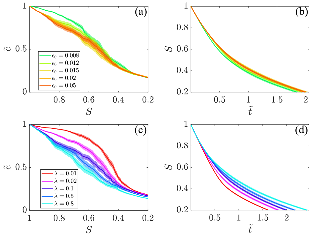
Figure 6: Drying curves (rate vs. saturation), and the temporal evolution of the saturation. The drying rate \tilde{e} decreases more gradually for lower \epsilon_0 values (a), mostly in the initial stages of drying, with a relatively limited effect on \tilde{t} (b). Similarly, \tilde{e} decreases more gradually for lower \lambda (c), resulting in shorter drying time \tilde{t} (d). Solid lines and shaded area represent the mean value and standard error, respectively, calculated from 20 realizations for each \lambda or \epsilon_0 value. We use a fixed value of \lambda = 0.1 for the simulations in a-b, and \epsilon_0 = 0.05 for c-d.
