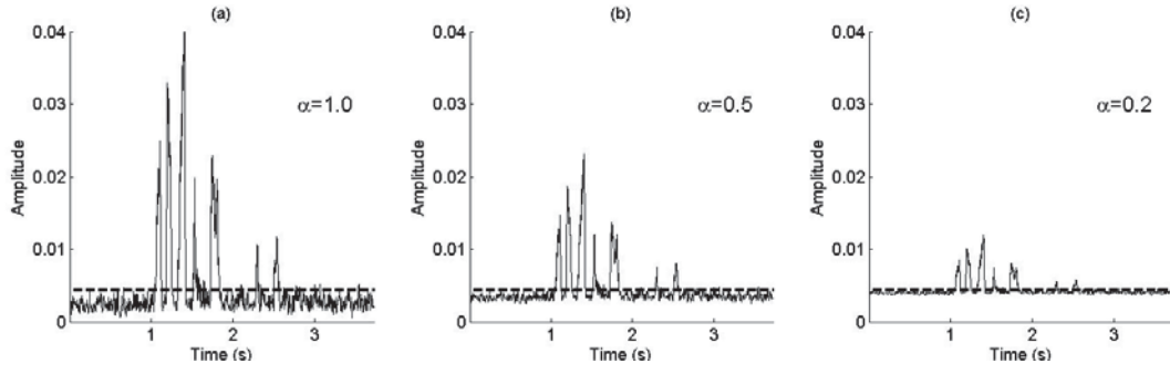
FIG 3. Example waveforms of compressed amplitude envelope with compression factor \alpha of values (a) 1.0, (b) 0.5, and (c) 0.2. The dashed line in each panel denotes the mean value of the amplitude envelope waveform.
