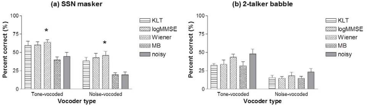
FIG 2. Sentence recognition scores for all conditions with and without noise reduction algorithms with (a) a -2-dB SNR SSN masker and (b) a 6-dB SNR 2TB masker. The error bars denote \pm 1 standard error of the mean. The asterisk denotes that the intelligibility score is significantly ( p < 0.01 ) larger than that in the noisy condition.
