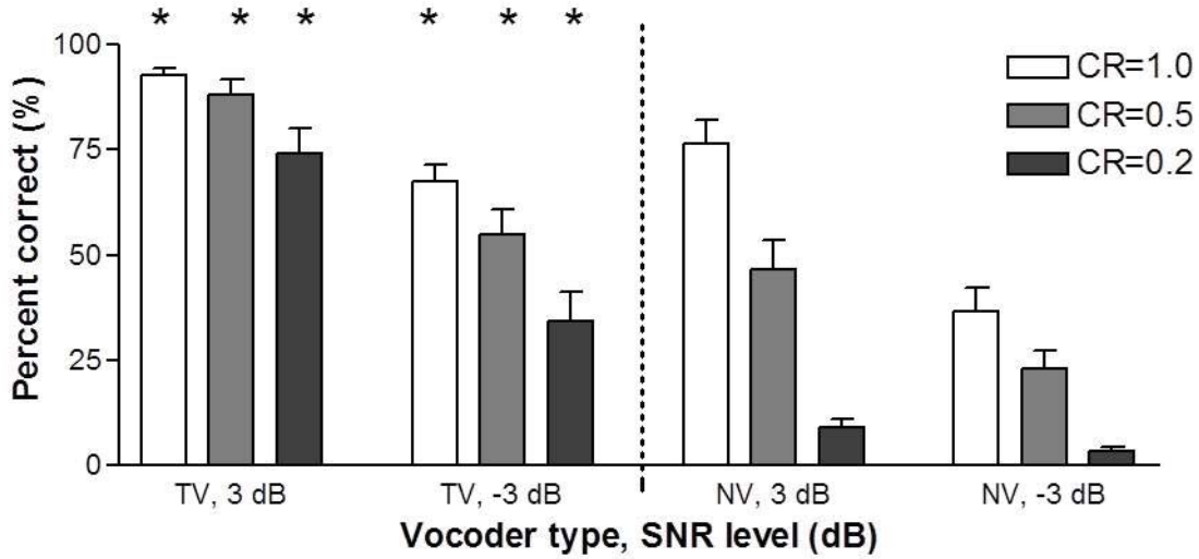
FIG 4. Sentence recognition scores for all test conditions. The error bars denote \pm 1 standard error of the mean. The asterisk denotes that the intelligibility score of tone-vocoded speech is significantly ( p < 0.005 ) larger than that of noise-vocoded speech.
