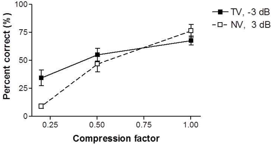
FIG 5. Sentence recognition scores for selected test conditions in Fig. 4. The solid and dashed lines show the scores for TV speech at -3 dB and NV speech at 3 dB, respectively. The error bars denote \pm 1 standard error of the mean.
