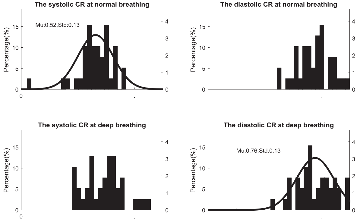
Figure 4. Histograms and fitted normal distributions of systolic and diastolic characteristic ratios (CRs) for both the normal and deep breathing conditions. (Mu: the mean of characteristic ratios; Std: the standard deviation of characteristic ratios).
