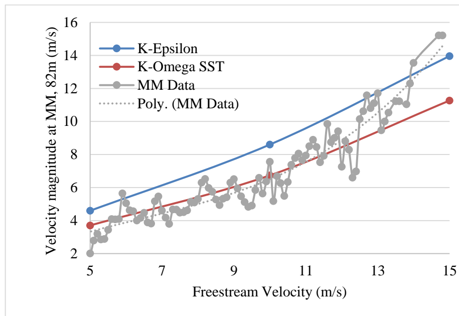
Figure 2. Comparison of turbulence models with met mast data.
