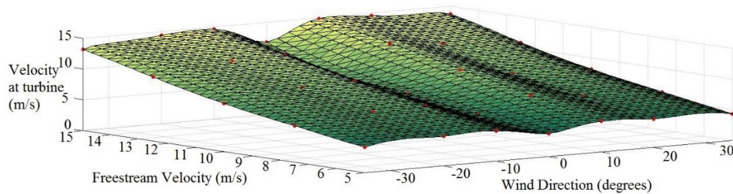
Figure 3. Prediction surface of RBF method for velocity magnitude at turbine 16
