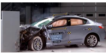
(a) 2016 Acura ILX small overlap impact test
