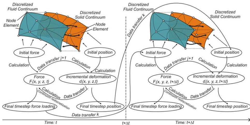
Fig. 5 FSI schematic
