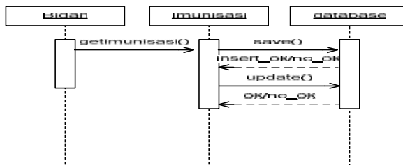
Gambar 9. Diagram Sequence catat data imunisasi
