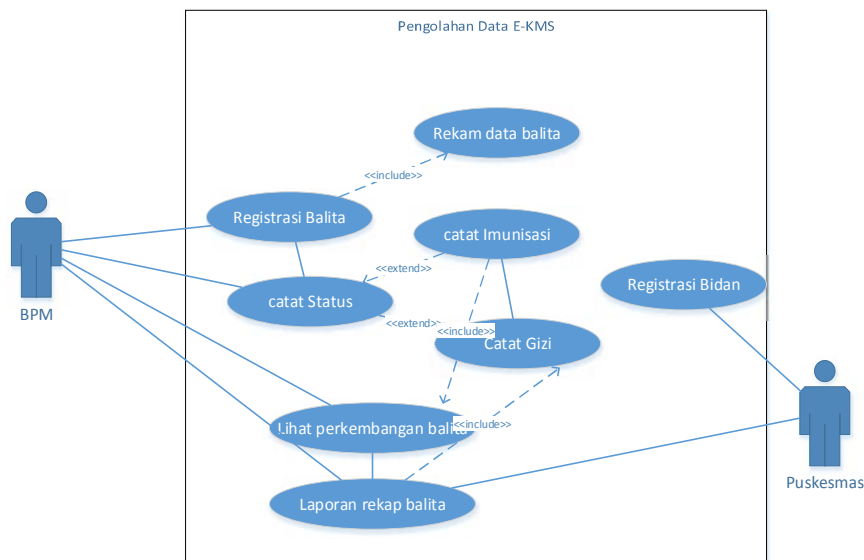
Gambar 7. Diagram usecase pengolahan data e-KMS
